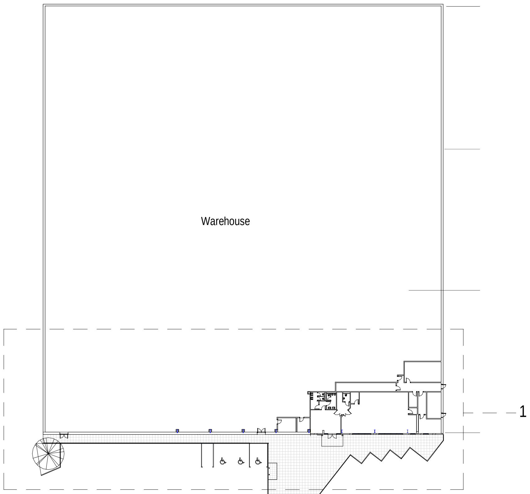
Level 0 (Ground Floor) Warehouse Existing Plan 1: 500 @ A1
