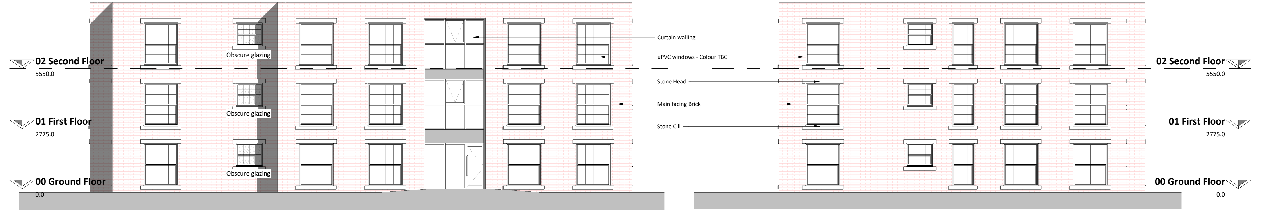
Front Elevation 1 : 100
