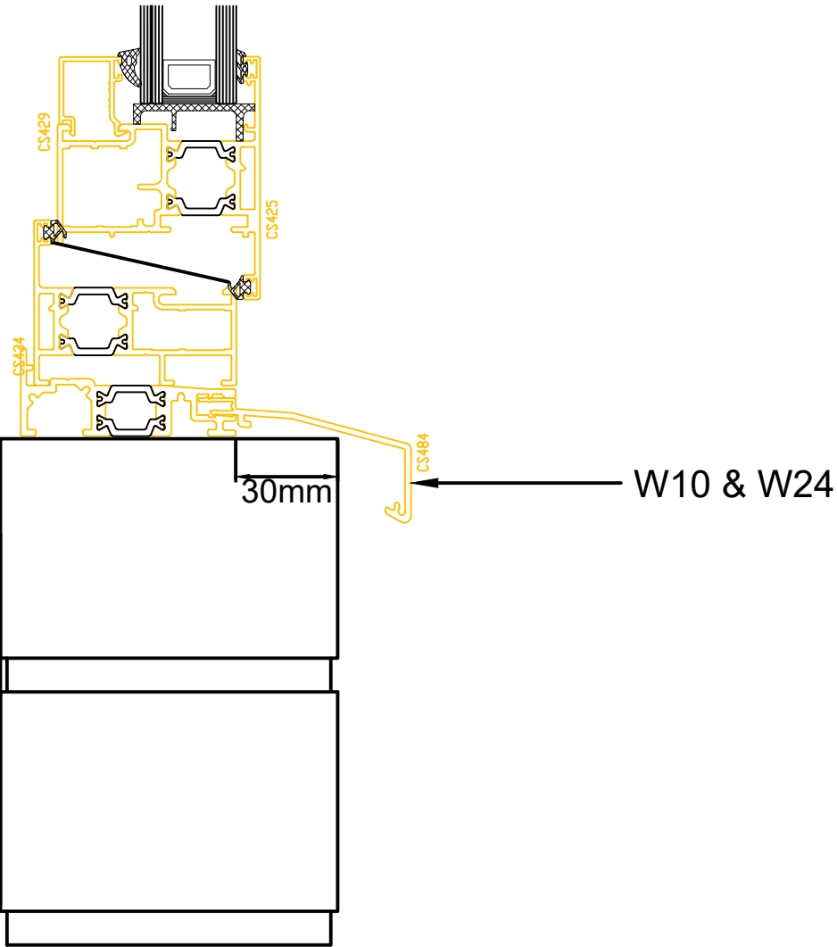
Standard Brick Cill Detail
