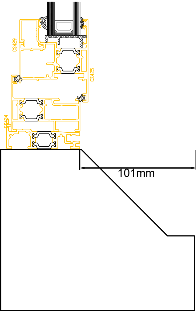
Stone Cill Detail
