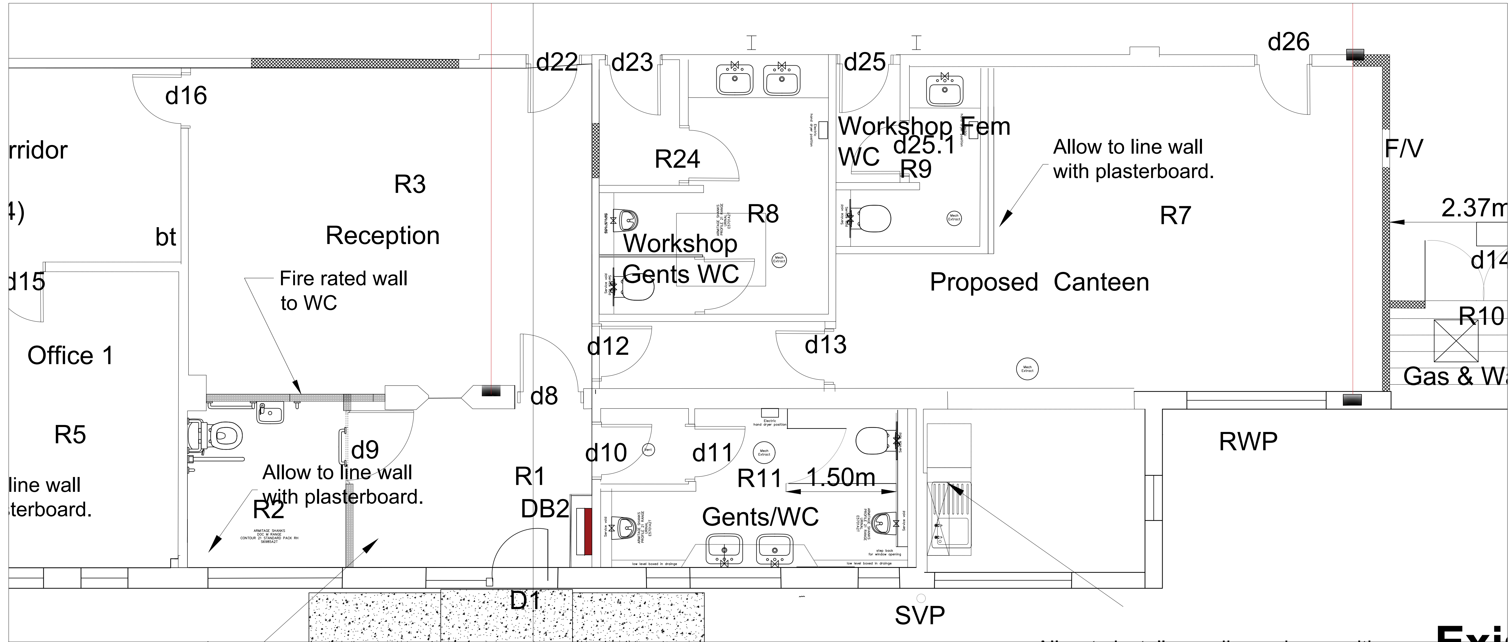
TOILET LAYOUT @ 1/30
