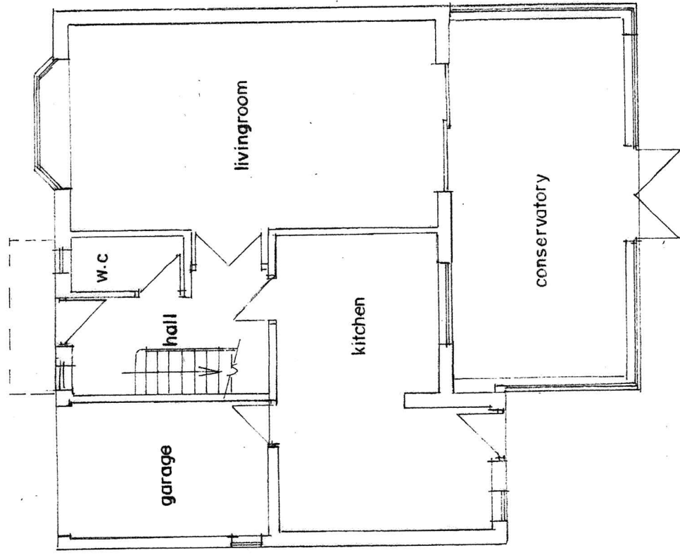
GROUND FLOOR PLAN (EXISTING)
