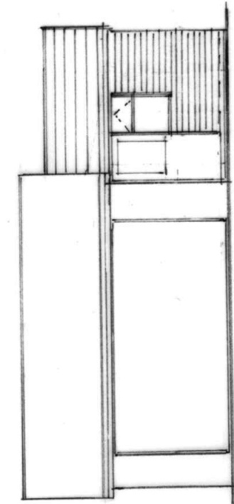
FRONT ELEVATION 'C' (PROPOSED)
