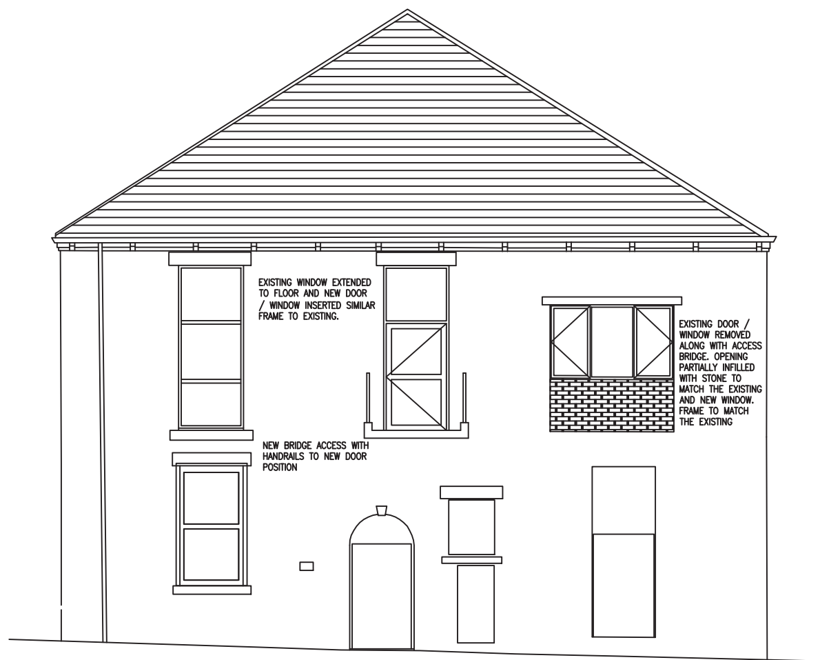
REAR ELEVATION
