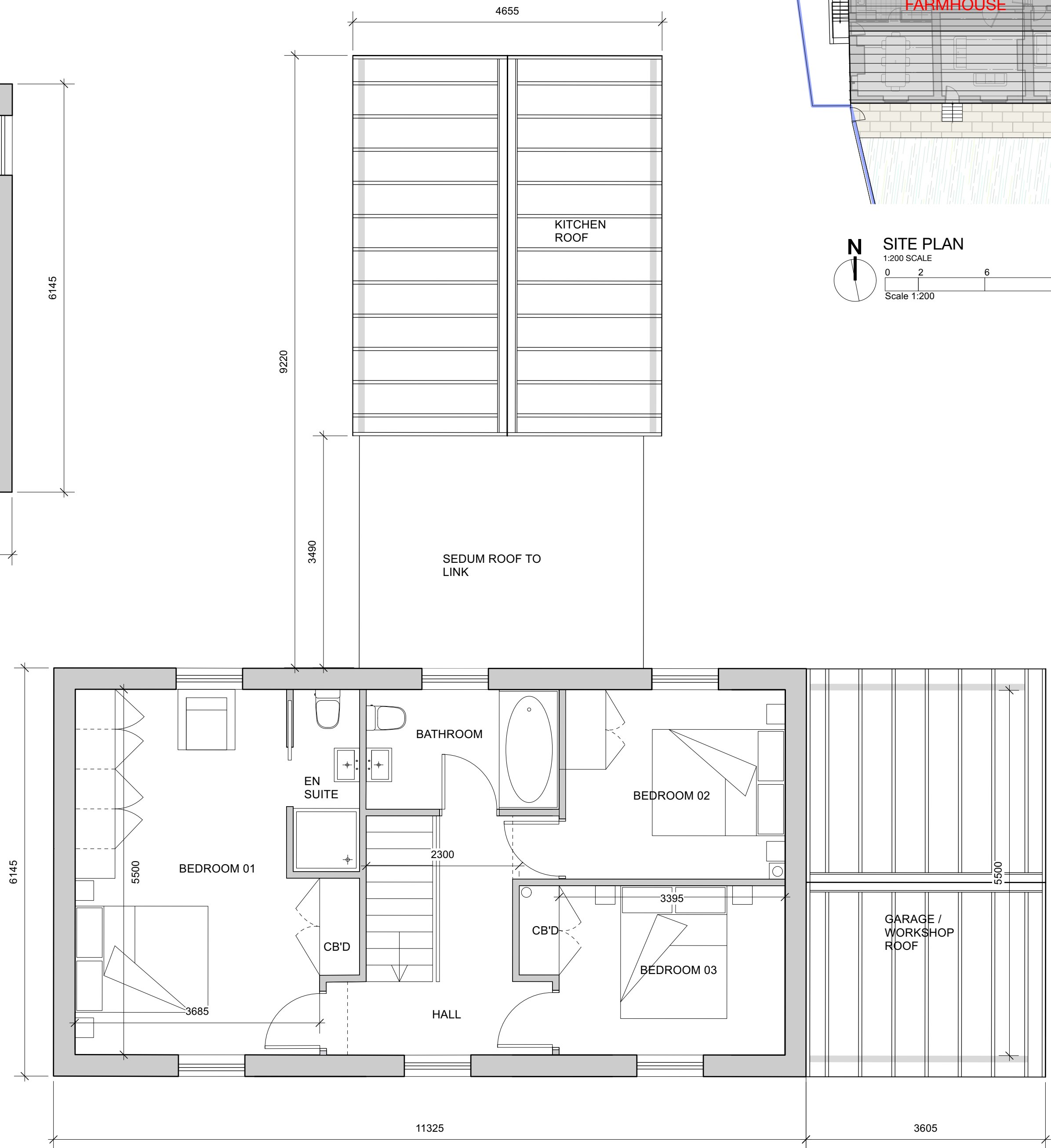
PROPOSED NEW DWELLING- FIRST FLOOR 1:50 SCALE 0 500 1,500 2,500mm Scale 1:50
