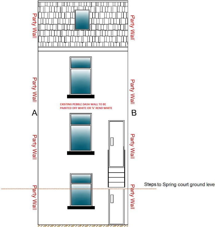
PROPOSED REAR ELEVATION 1:50 @ A1
