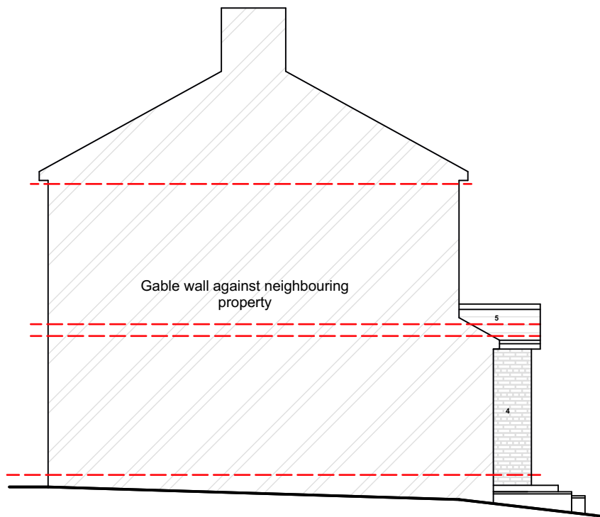
PROPOSED GA SIDE ELEVATION 2 @1:100
