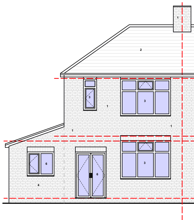
PROPOSED GA REAR ELEVATION @1:100
