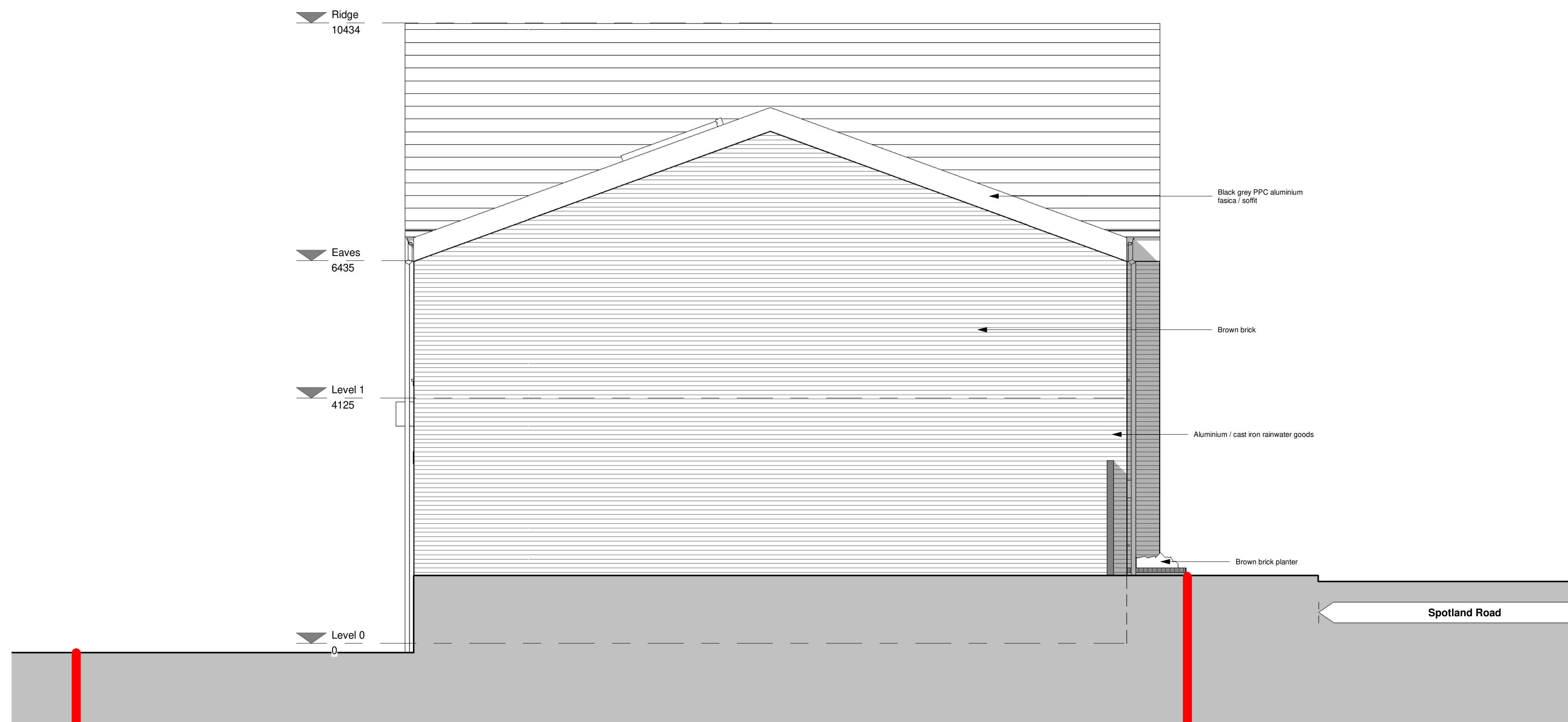
2 Proposed East Elevation
