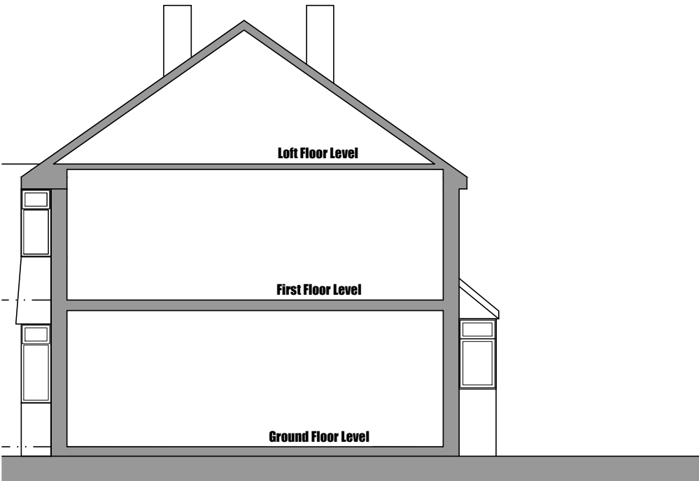
West Facing Side Elevational Section
