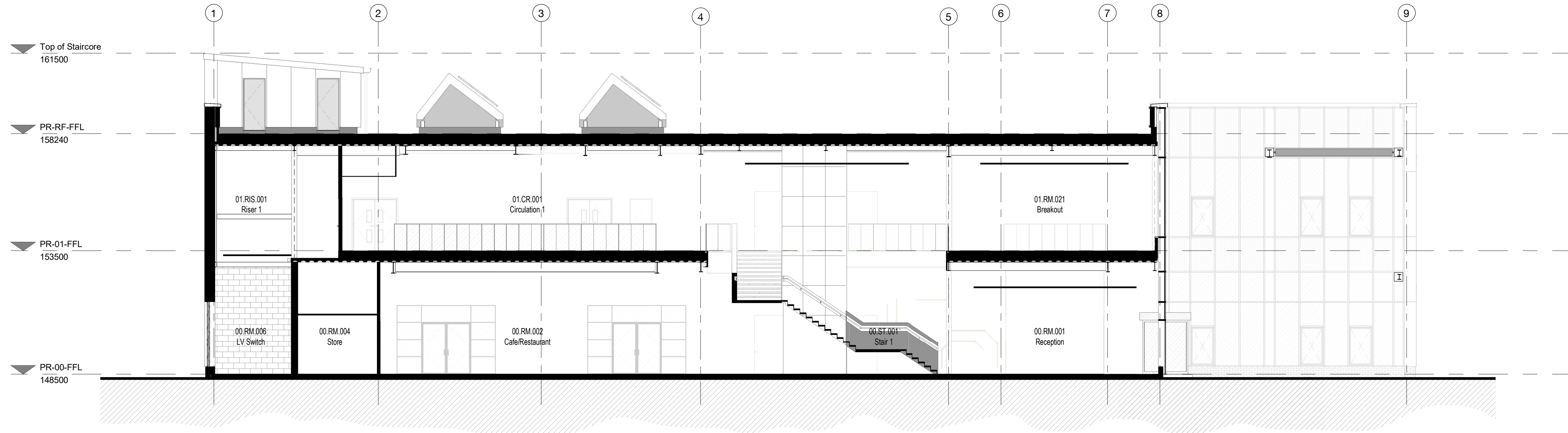
GA Section 3
