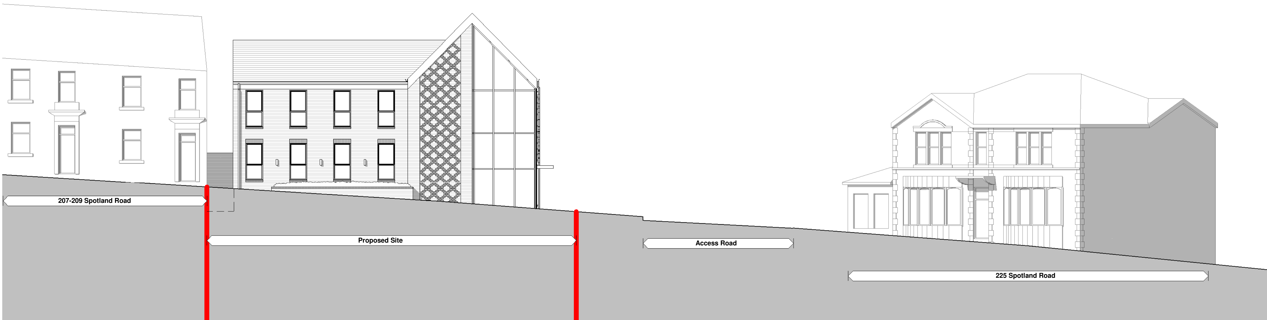
2 Proposed North Streetscene Elevation 1 : 100
