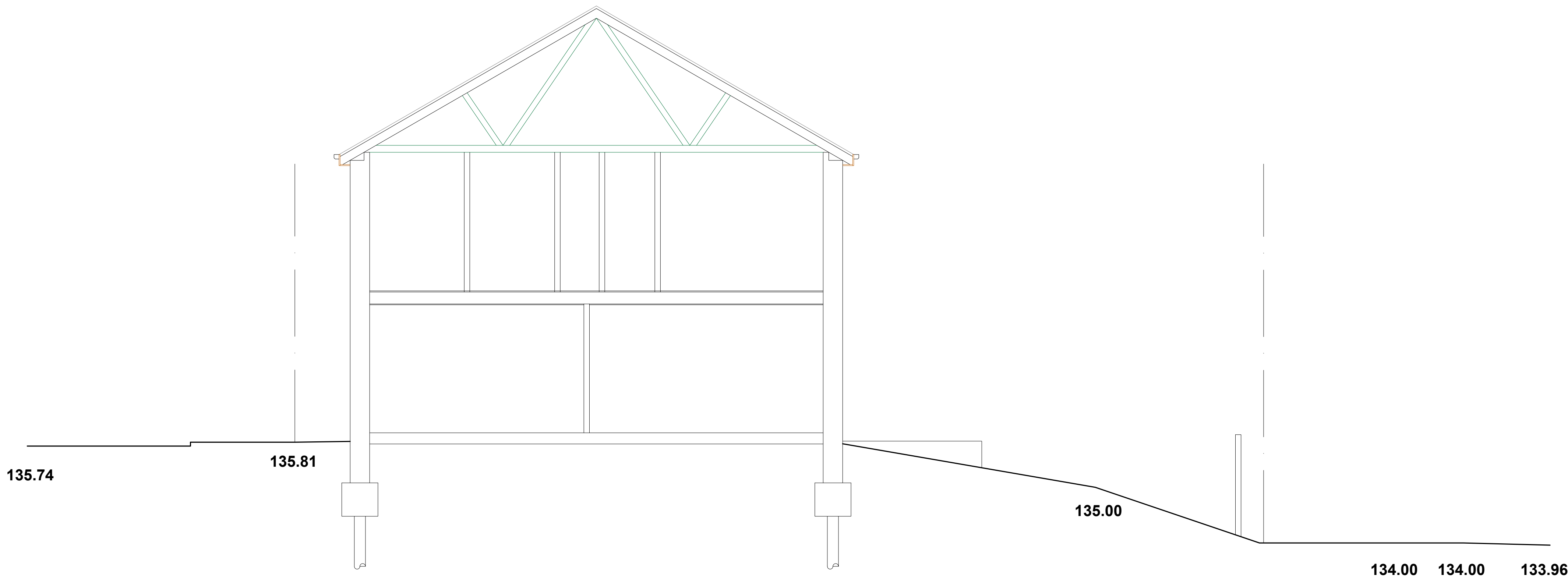
PROPOSED SITE SECTION X - X
