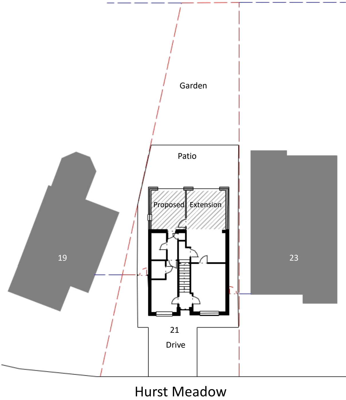
PROPOSED SITE PLAN (1:200)
