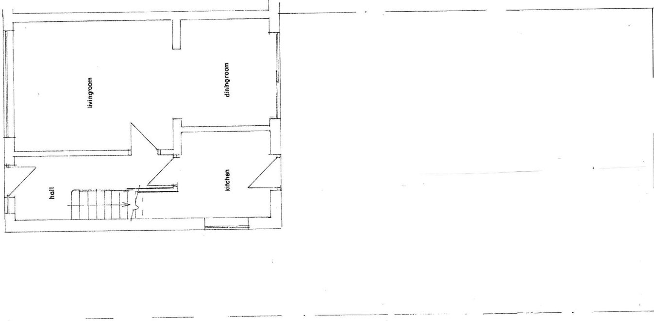
G.F. PLAN (EXISTING)
