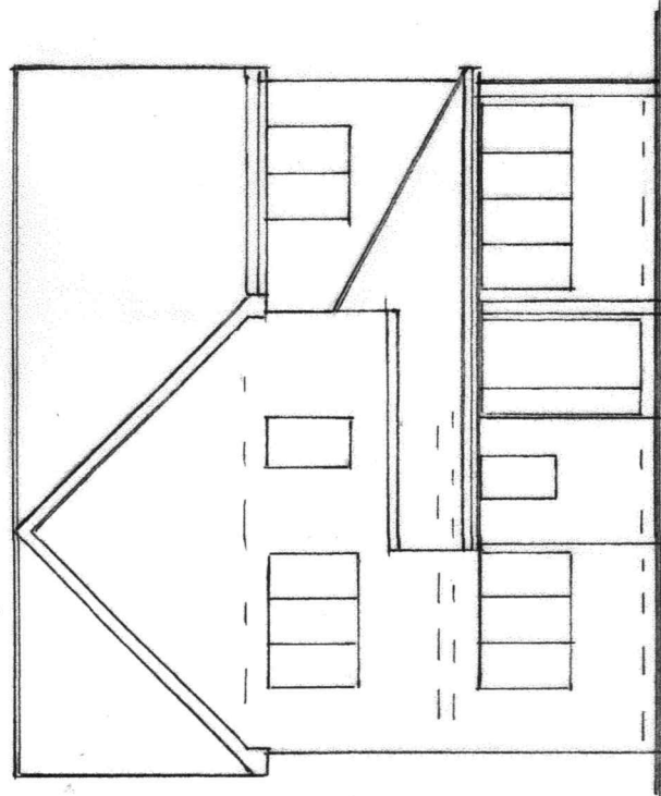
FRONT ELEVATION (EXISTING)
