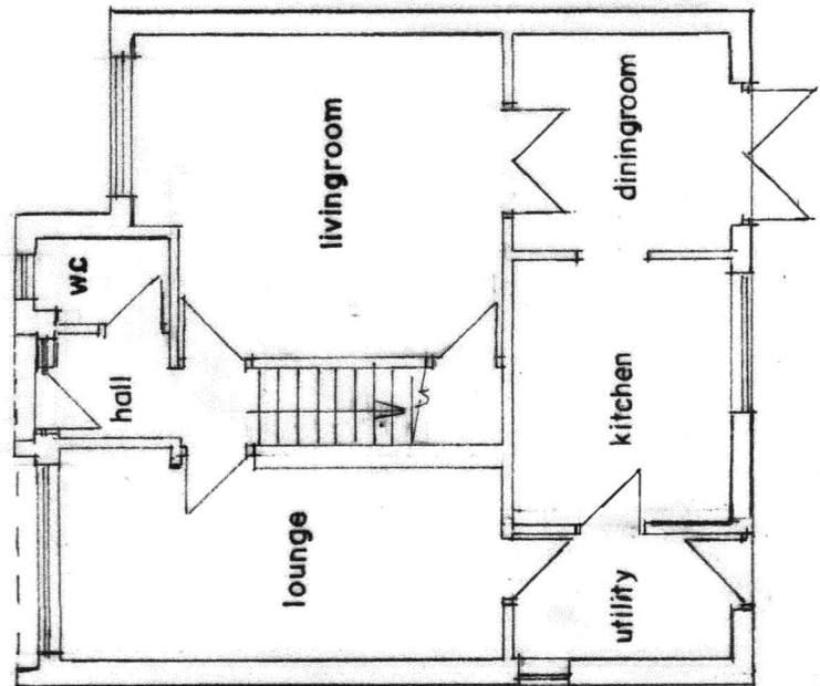
GROUND FLOOR PLAN (EXISTING)
