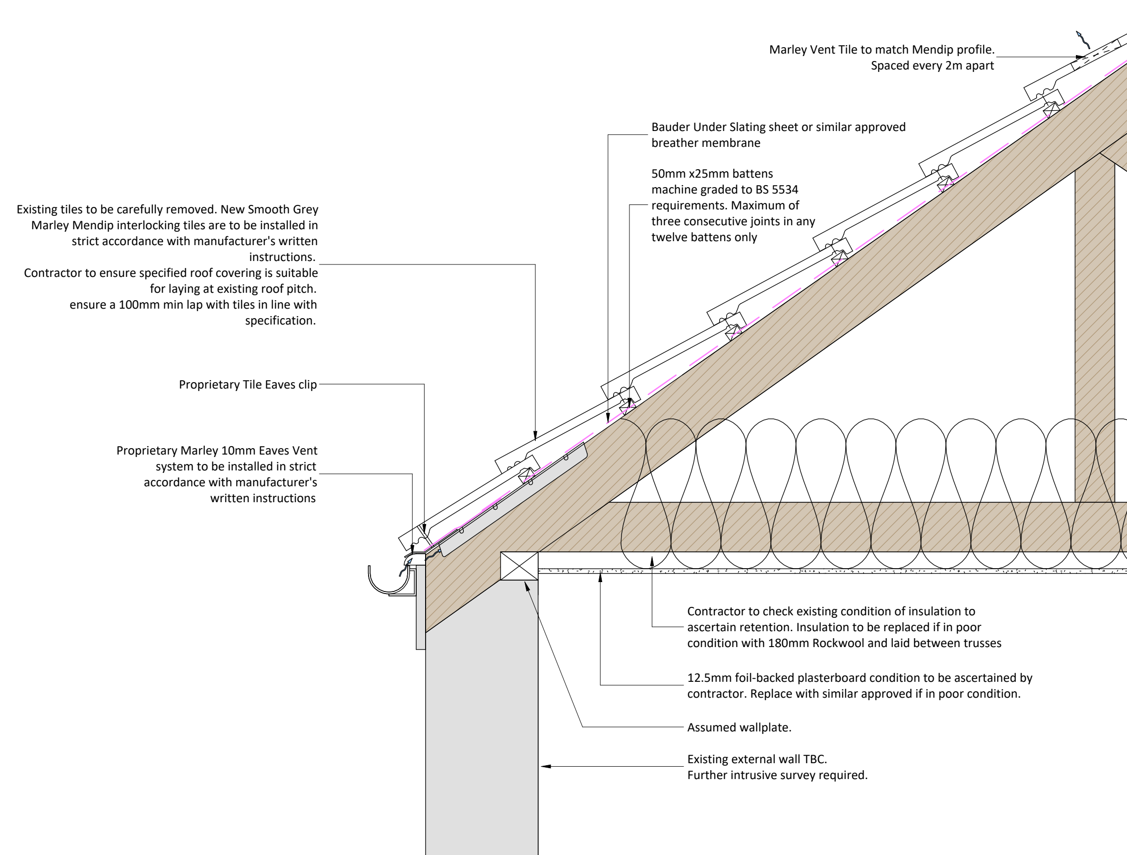
Roof Valley Gutter Detail - Detail A
