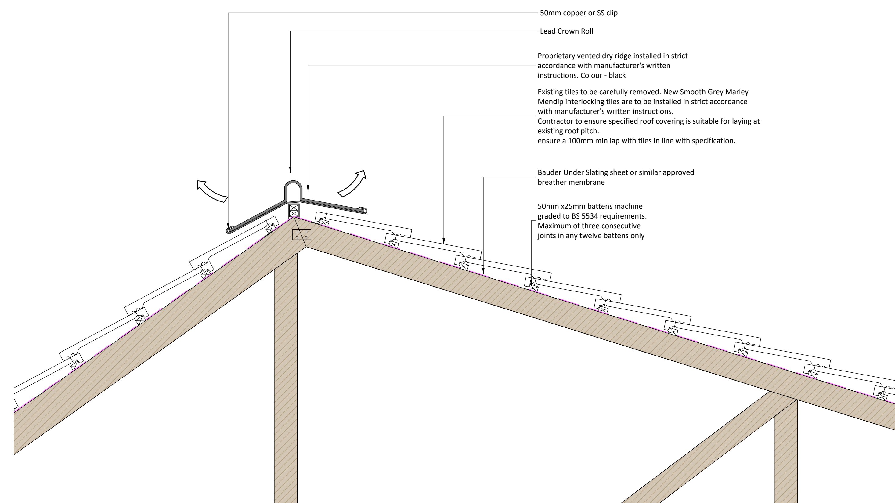
Roof Valley Gutter Detail - Detail B
