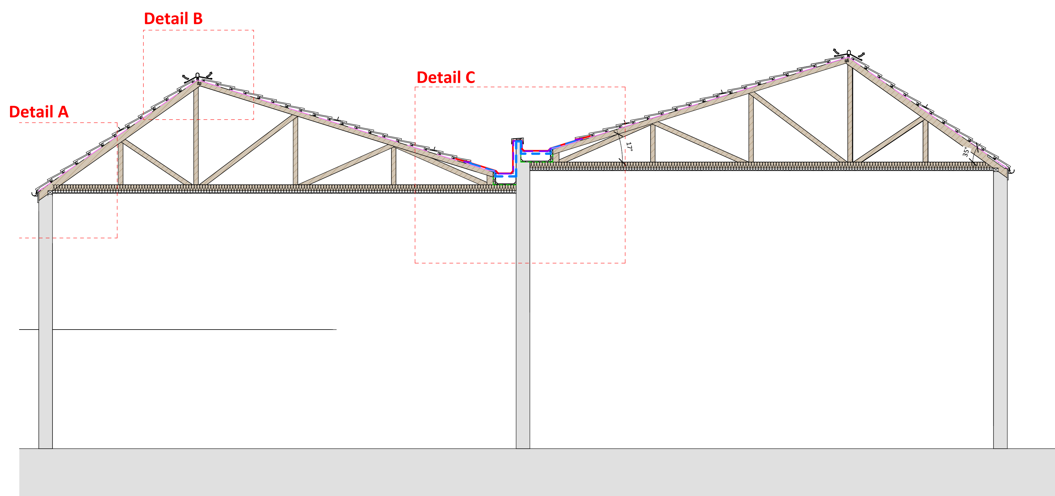
Roof Valley Gutter Detail - Proposed Section AA
