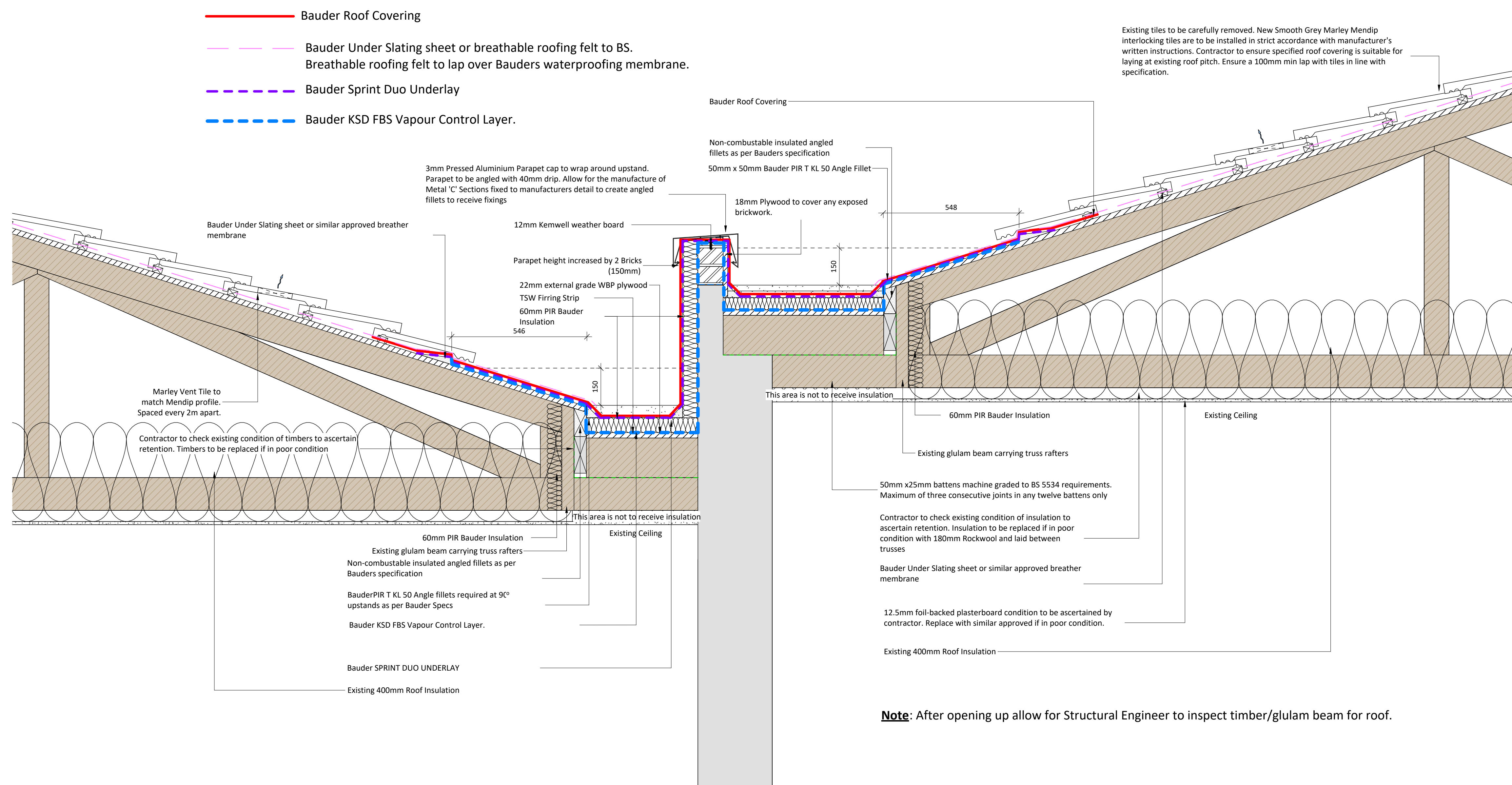
Roof Valley Gutter Detail - Detail C
