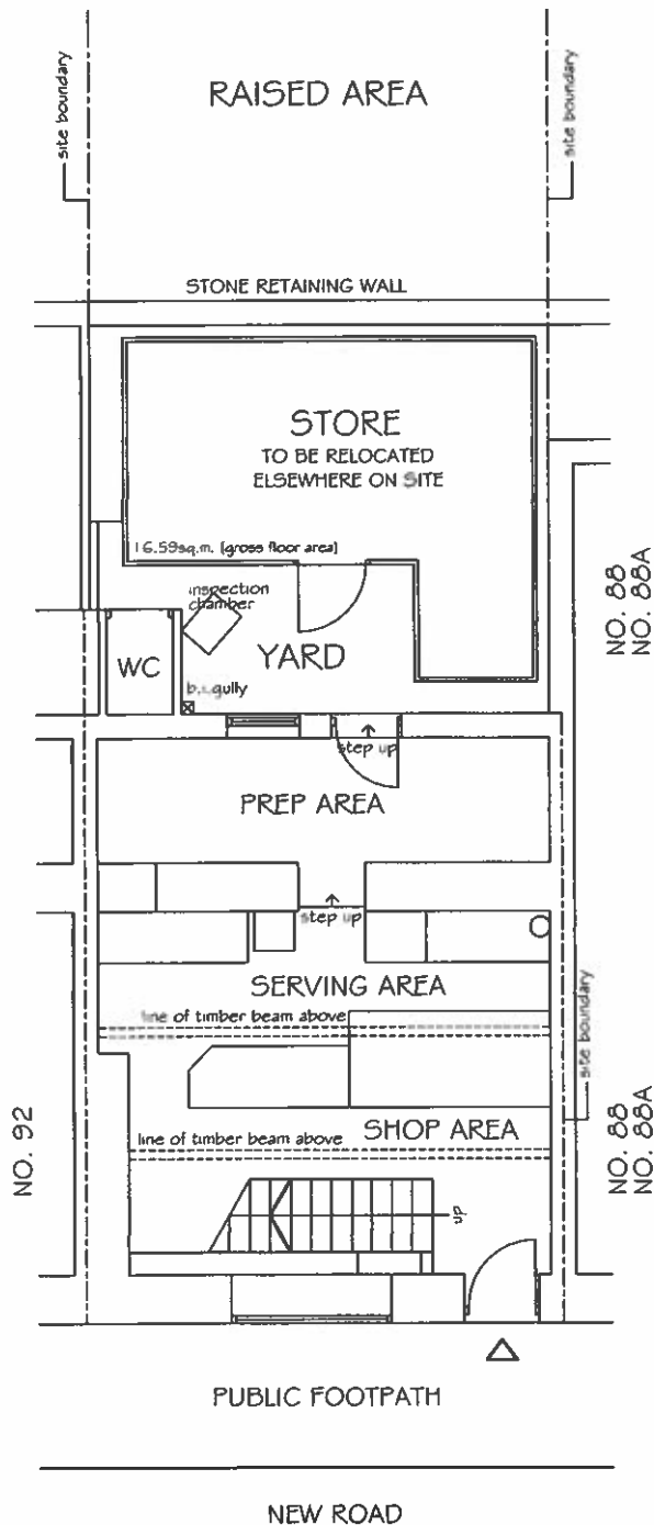
EXISTING GROUND FLOOR 1:100 LAYOUT
