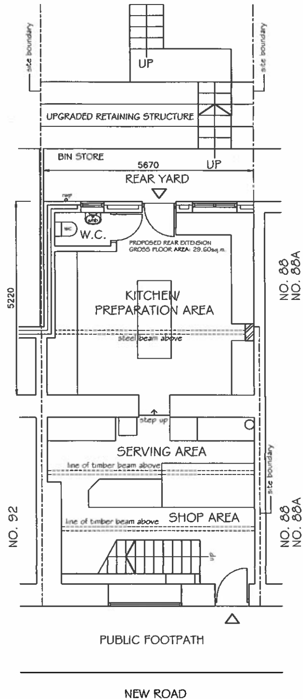
PROPOSED GROUND FLOOR 1:100 LAYOUT
