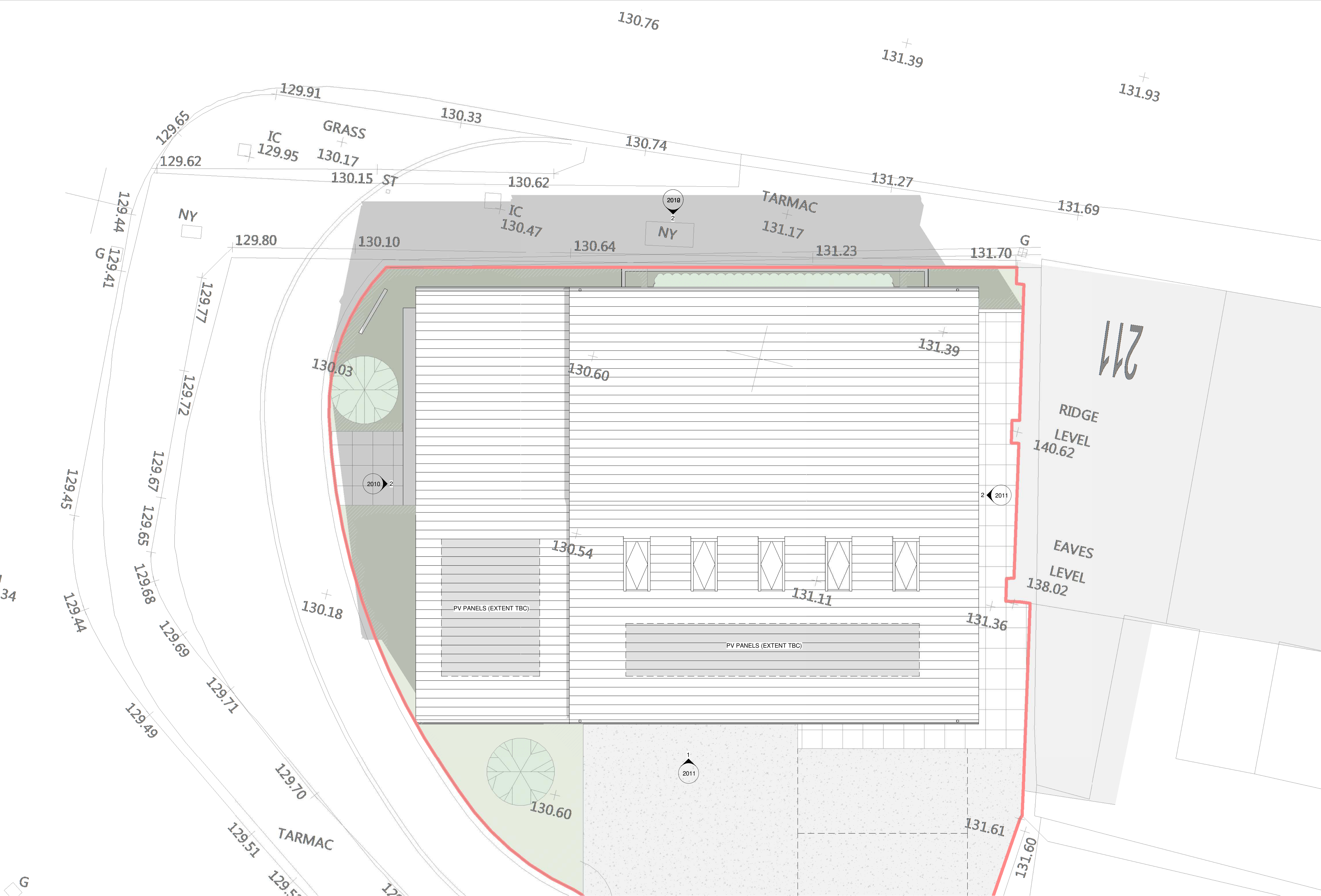
1 Proposed Roof Level 1:50
