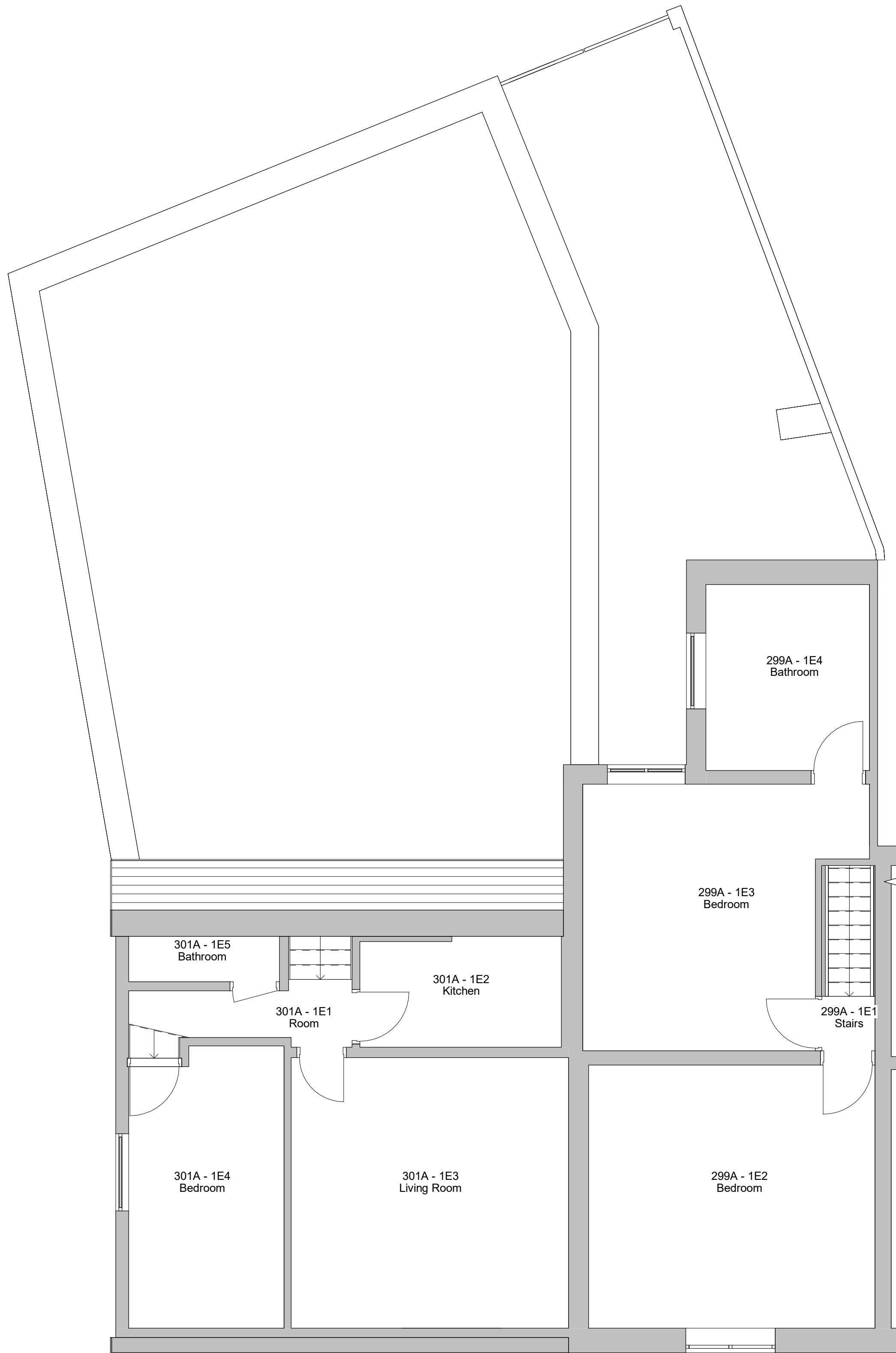
2 Level 1 - Proposed 1 : 50
