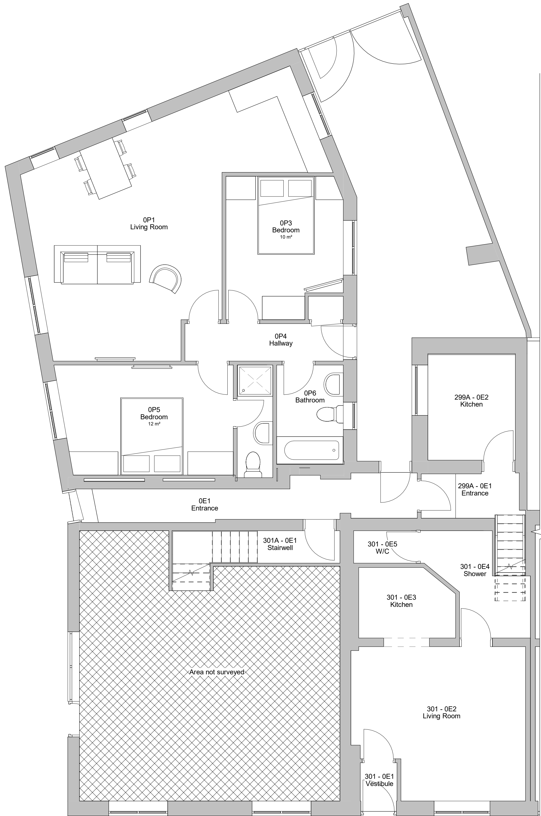
1 Level 0 New - Proposed 1 : 50
