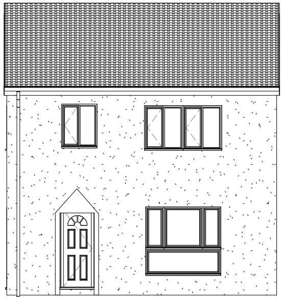
Existing Front 1 : 100
