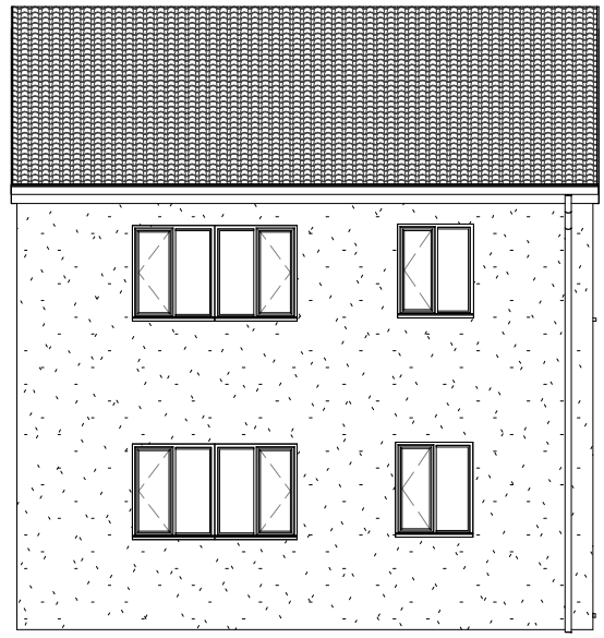
Existing Rear 1 : 100
