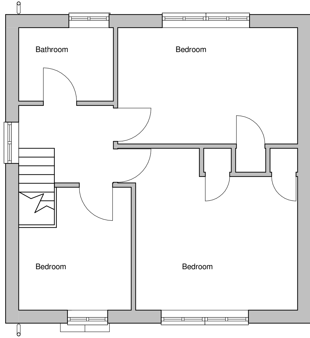
Existing First Floor 1 : 50
