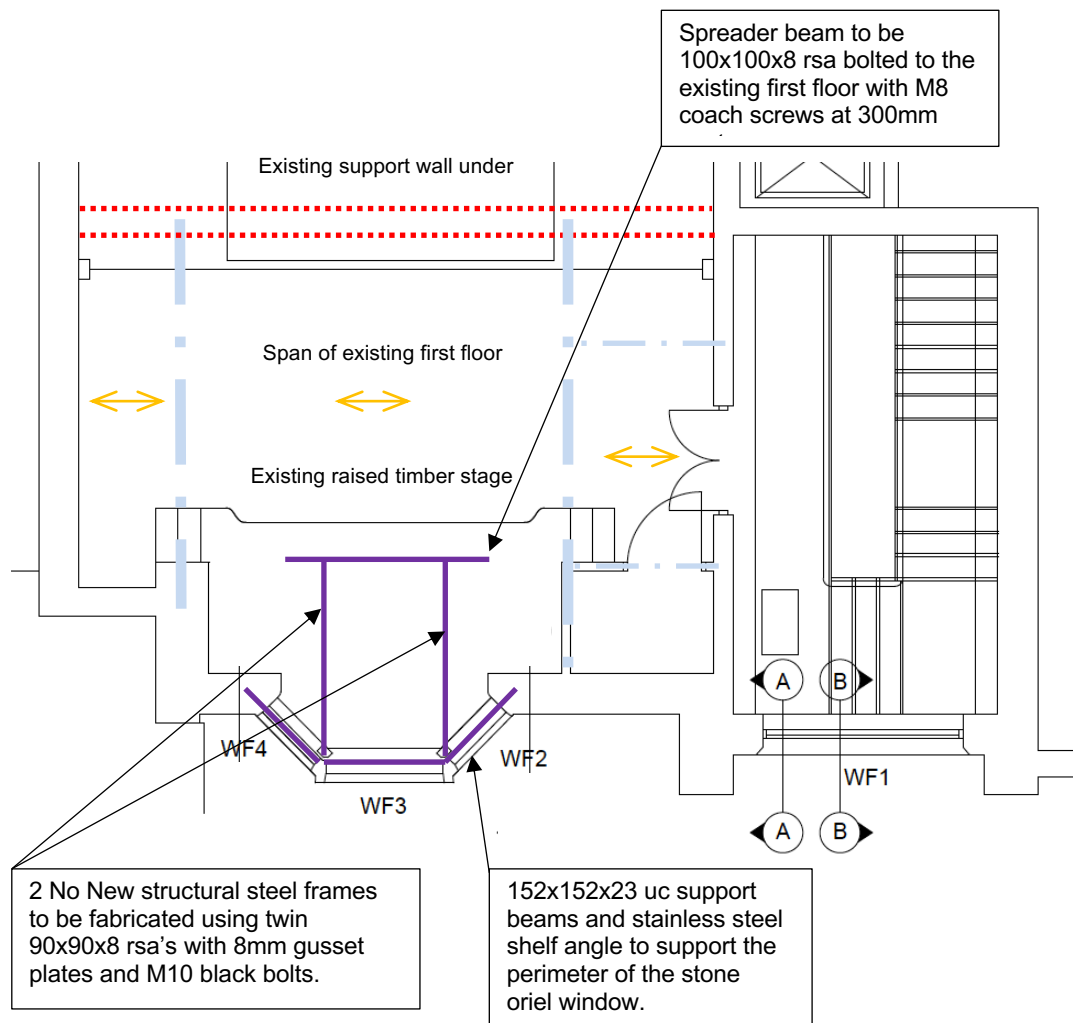
First Floor - Part Plan with Existing Beams Under
