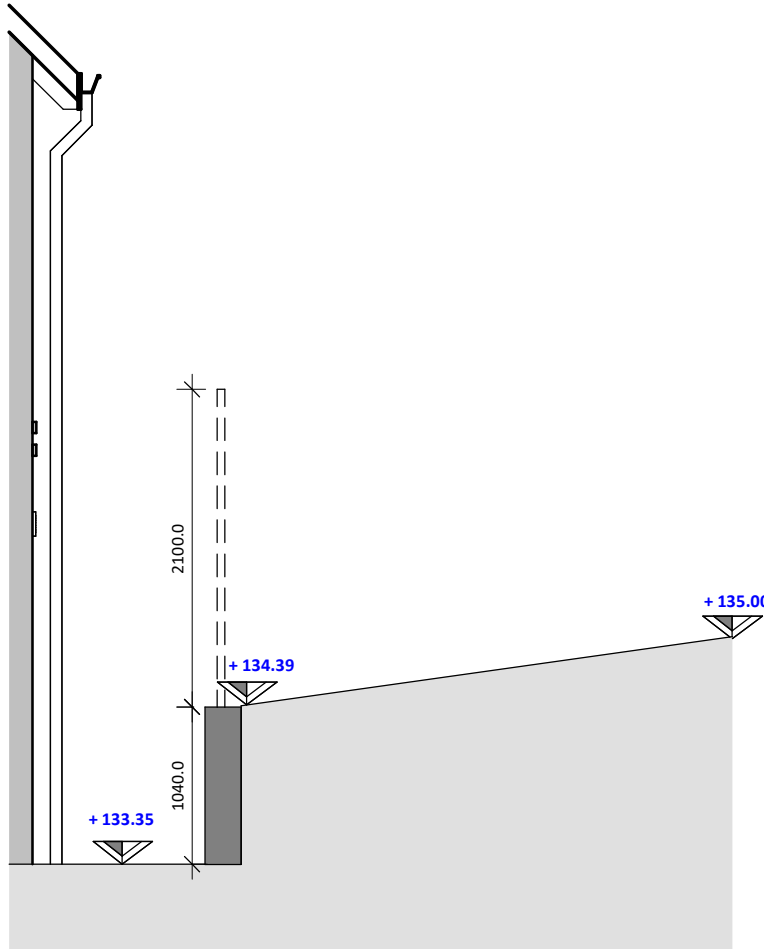
Plot 16 Side Section 1 1 : 50
