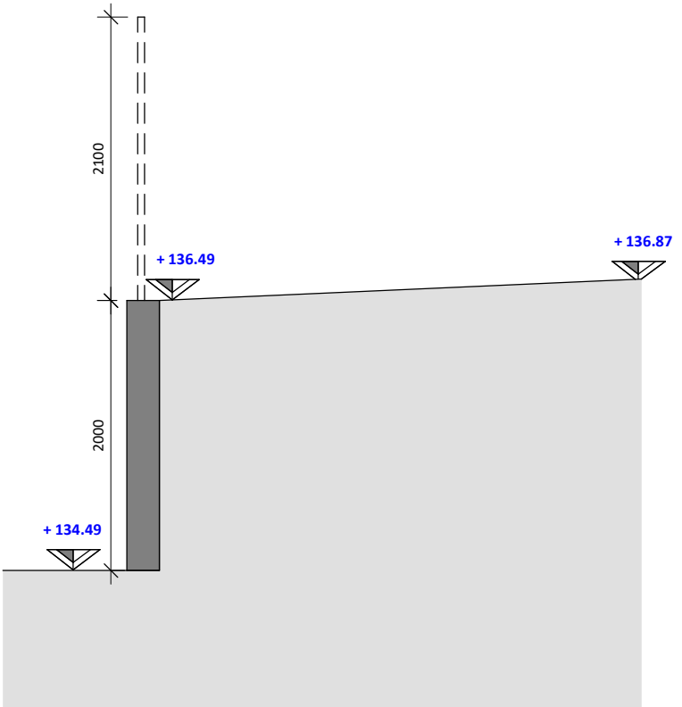
Plot 16 Side Section 3 1 : 50
