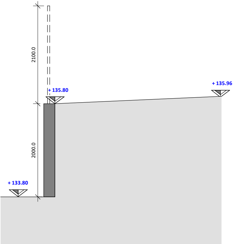
Plot 16 Side Section 2 1 : 50
