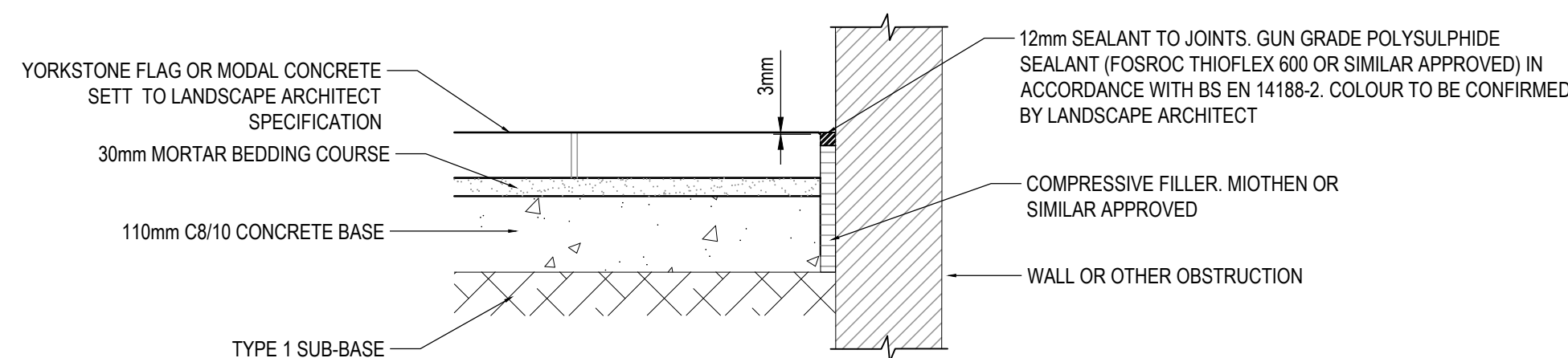
ISOLATION JOINT 1:10
