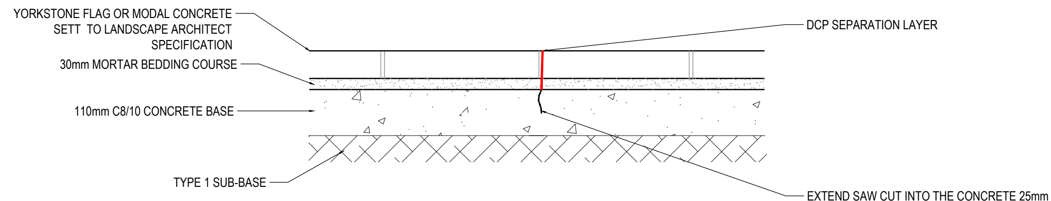
TYPICAL CONTRACTION JOINT 1:10
