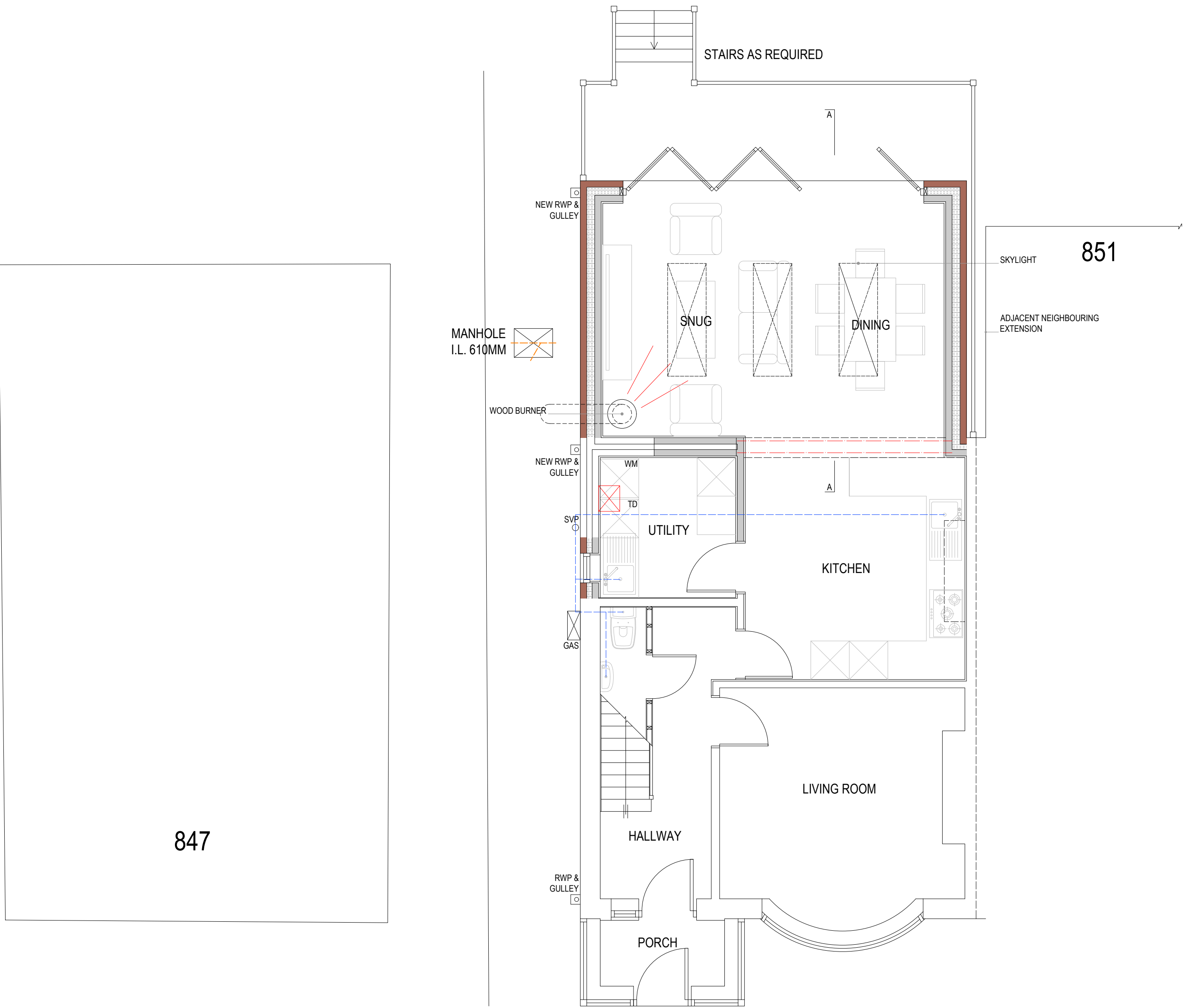
PROPOSED GROUND
