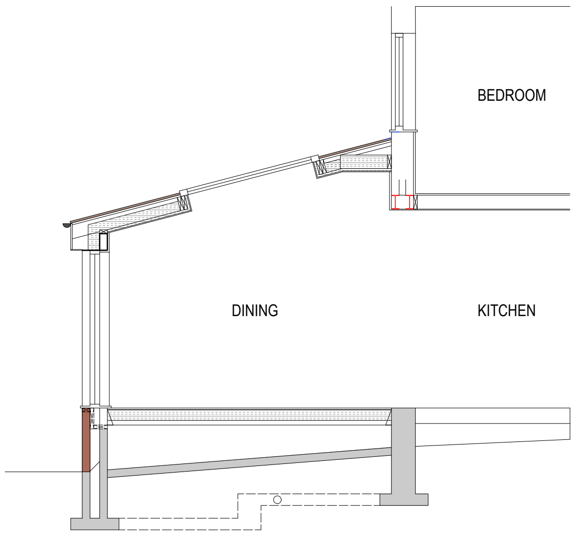
PROPOSED SECTION A-A
