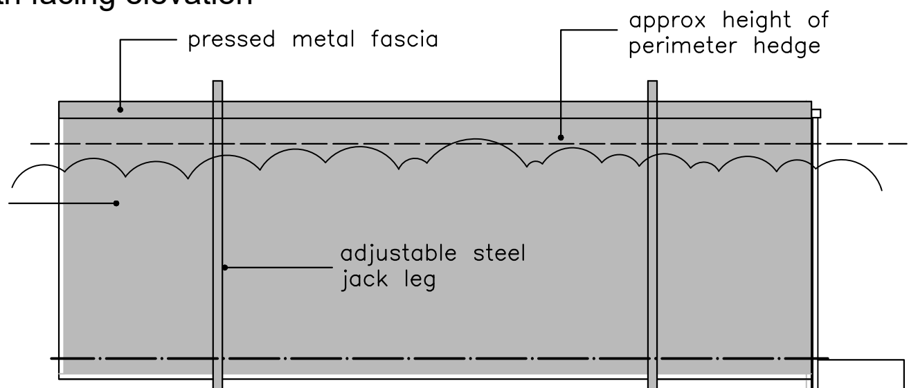
south facing elevation
