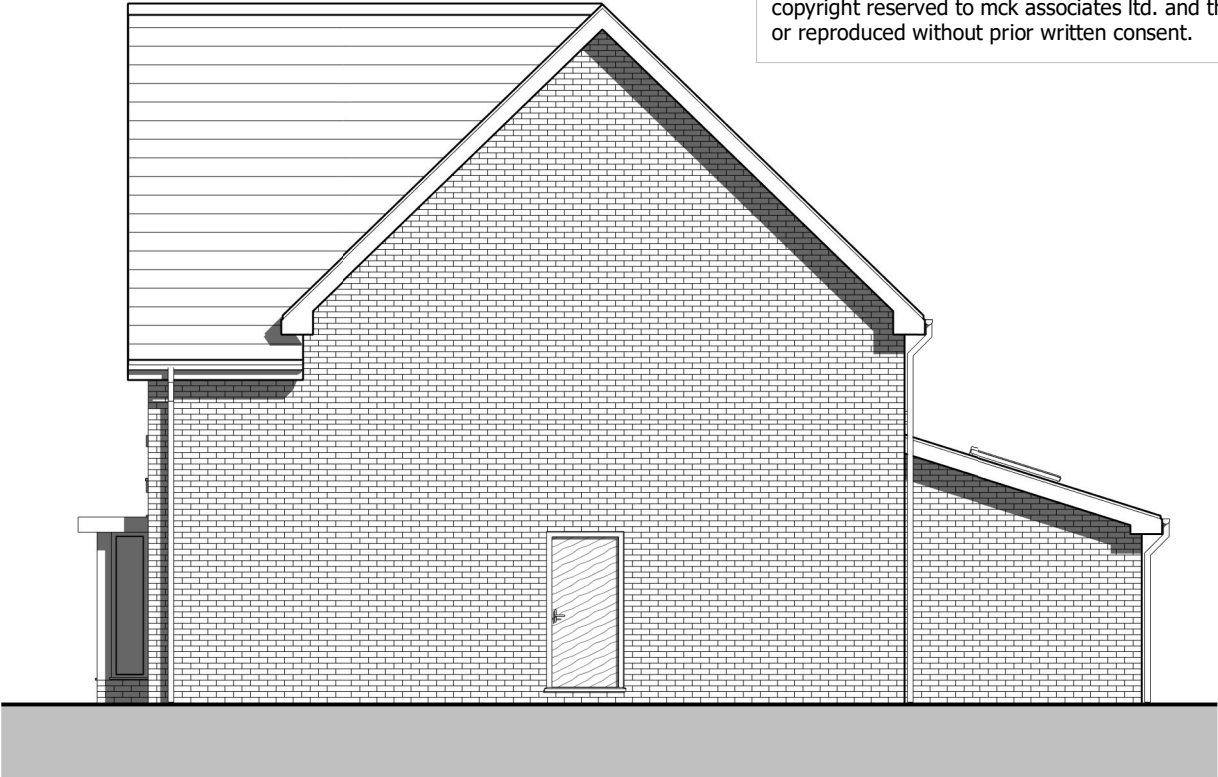
SIDE ELEVATION
