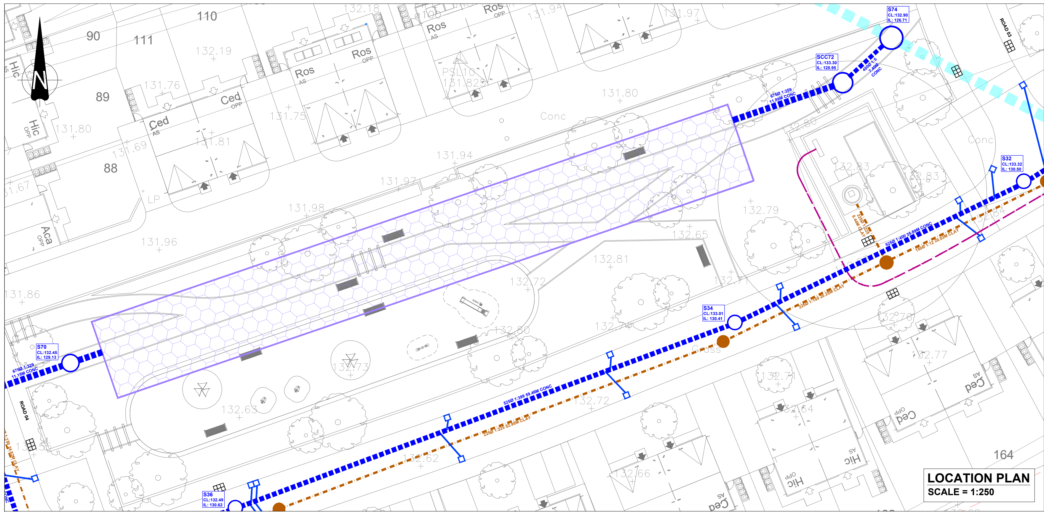
ONLINE 'POLYSTORM - XTRA - PSM3' (OR SIMILAR APPROVED) CELLULAR STORAGE TANK & CATCHPIT CHAMBER - TYPICAL CONSTRUCTION DETAIL
