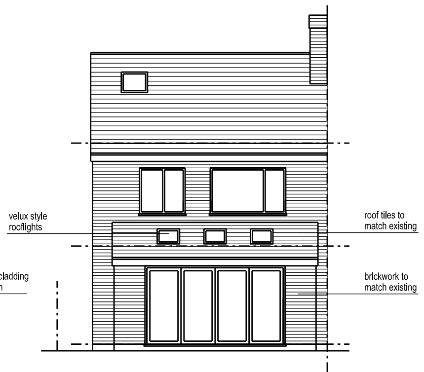
South Elevation
