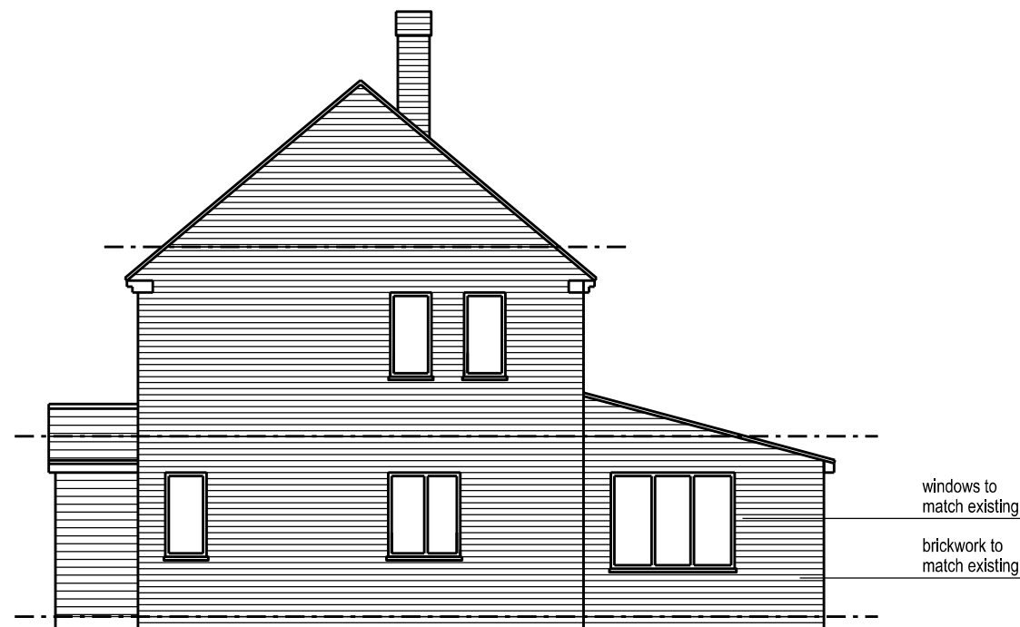
West Elevation
