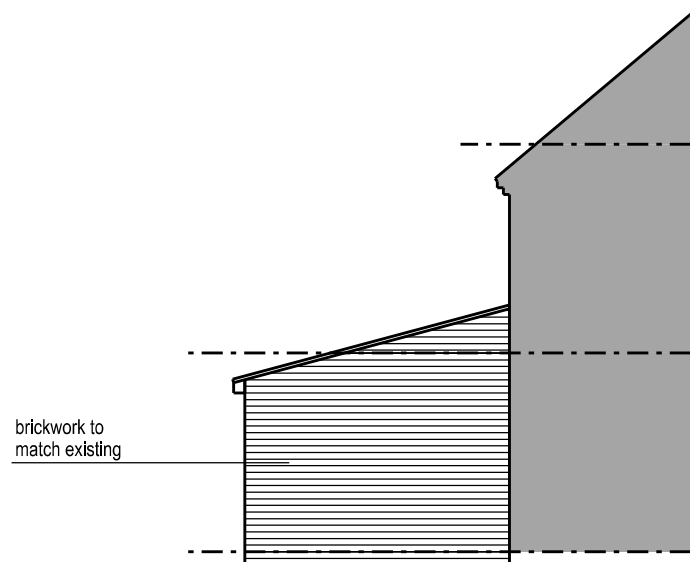
East Elevation
