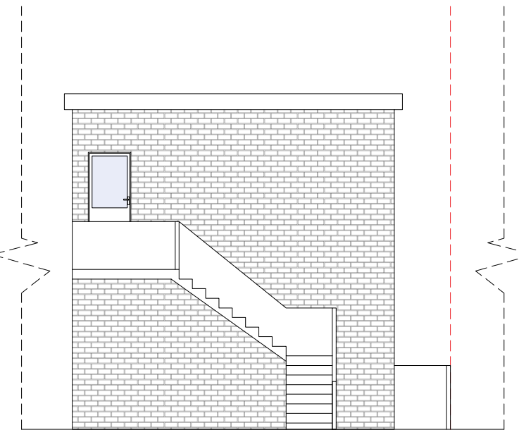
Proposed West Elevation (No Proposed Change)
