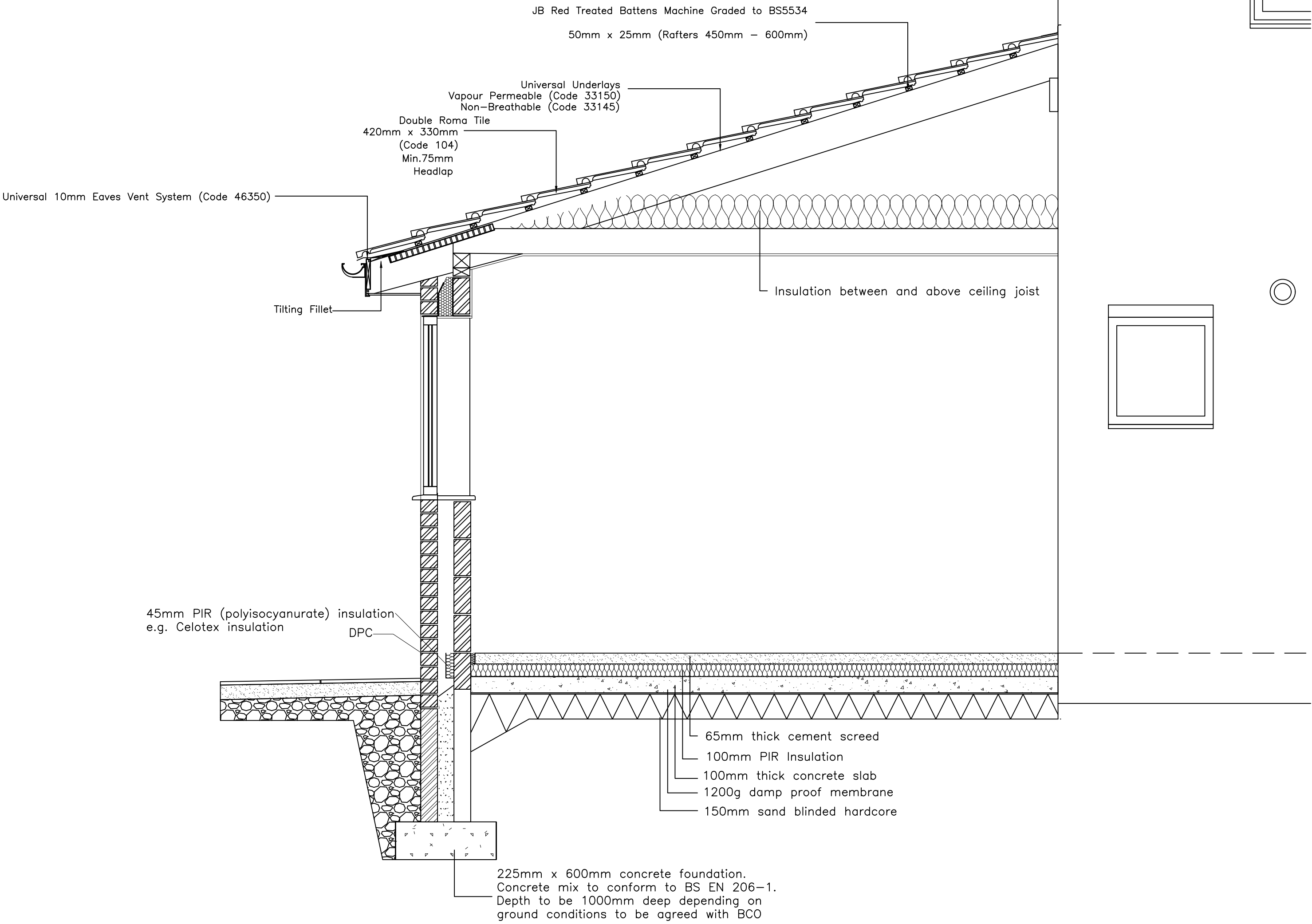
SECTION A-1
