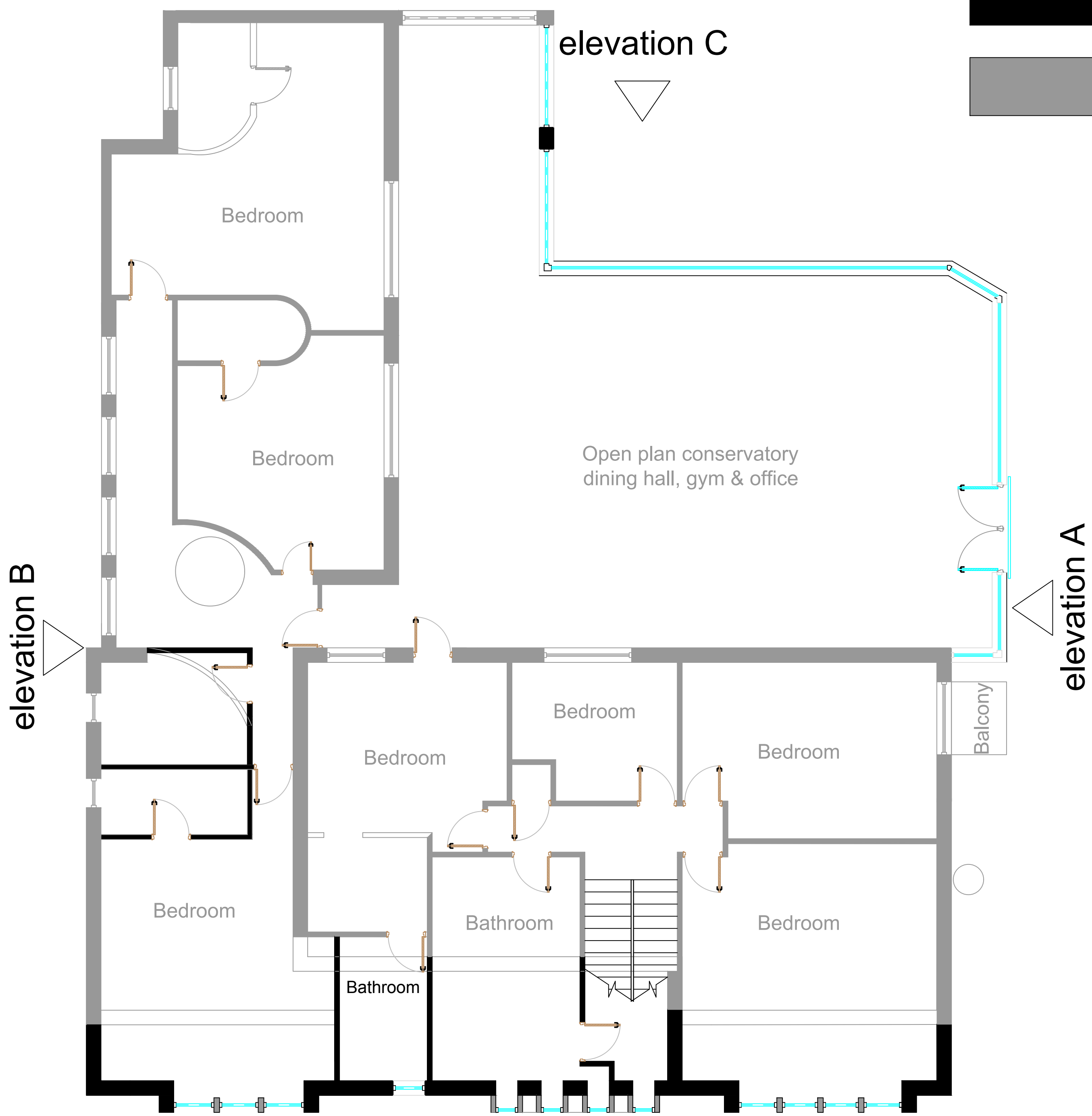
PROPOSED FIRST FLOOR PLAN 1:50 @ A1
