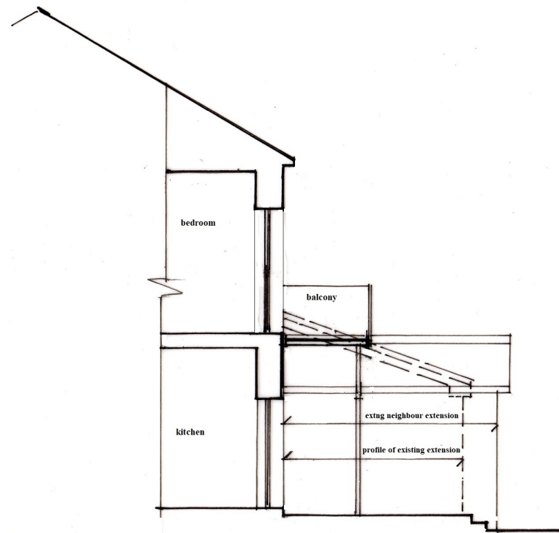
existing section
