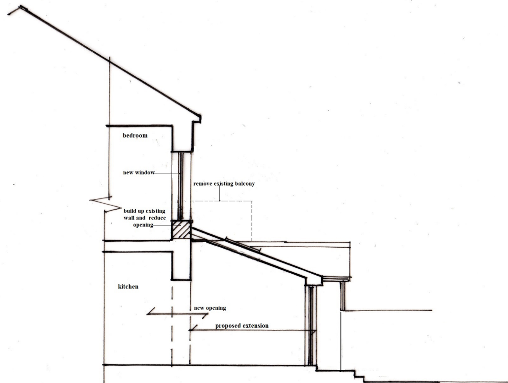
proposed section
