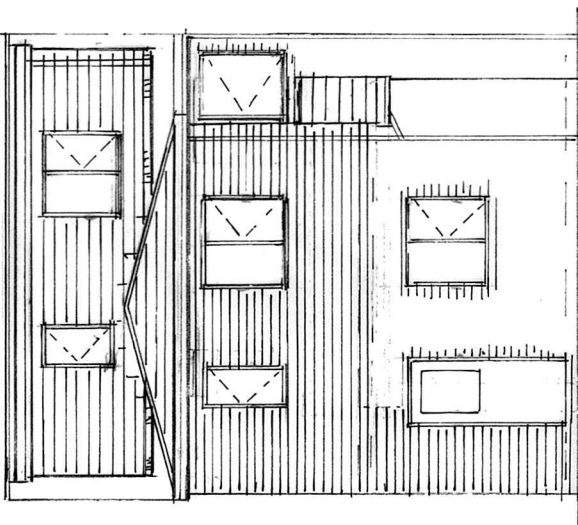
REAR ELEVATION (PROPOSED)
