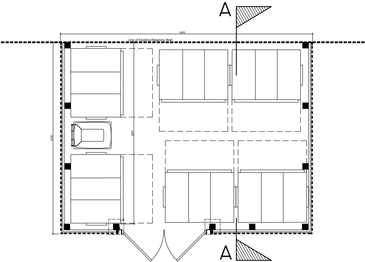
BIN STORE PLAN G.A
