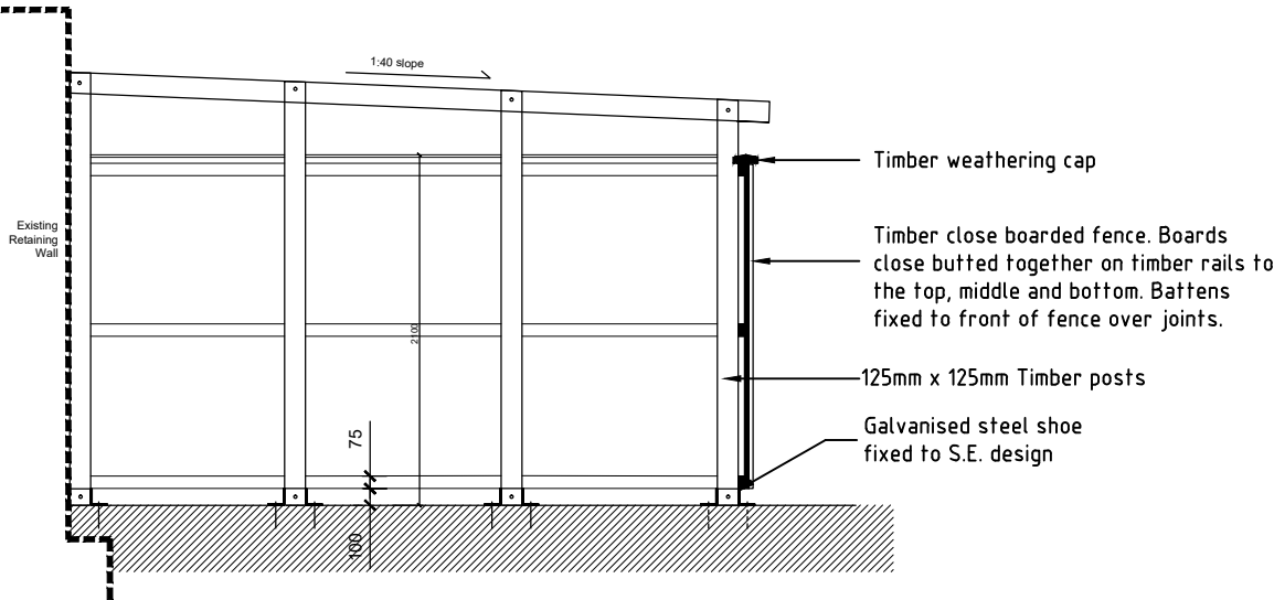
BIN STORE SECTION A-A
