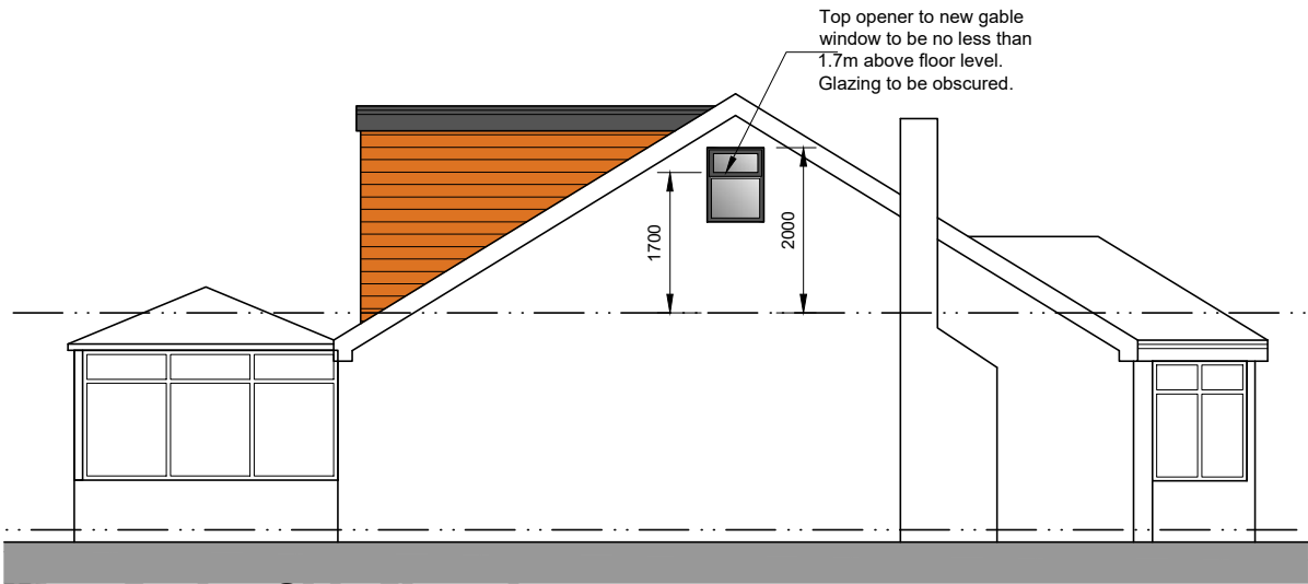
West Facing Side Elevation
