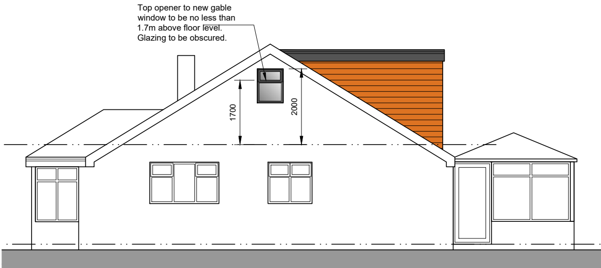
East Facing Side Elevation
