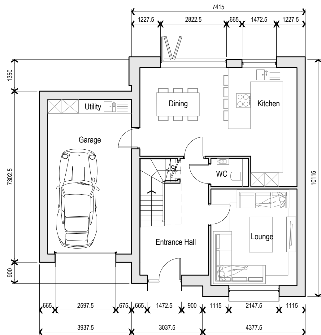
PROPOSED GROUND FLOOR PLAN 1:100@A3
