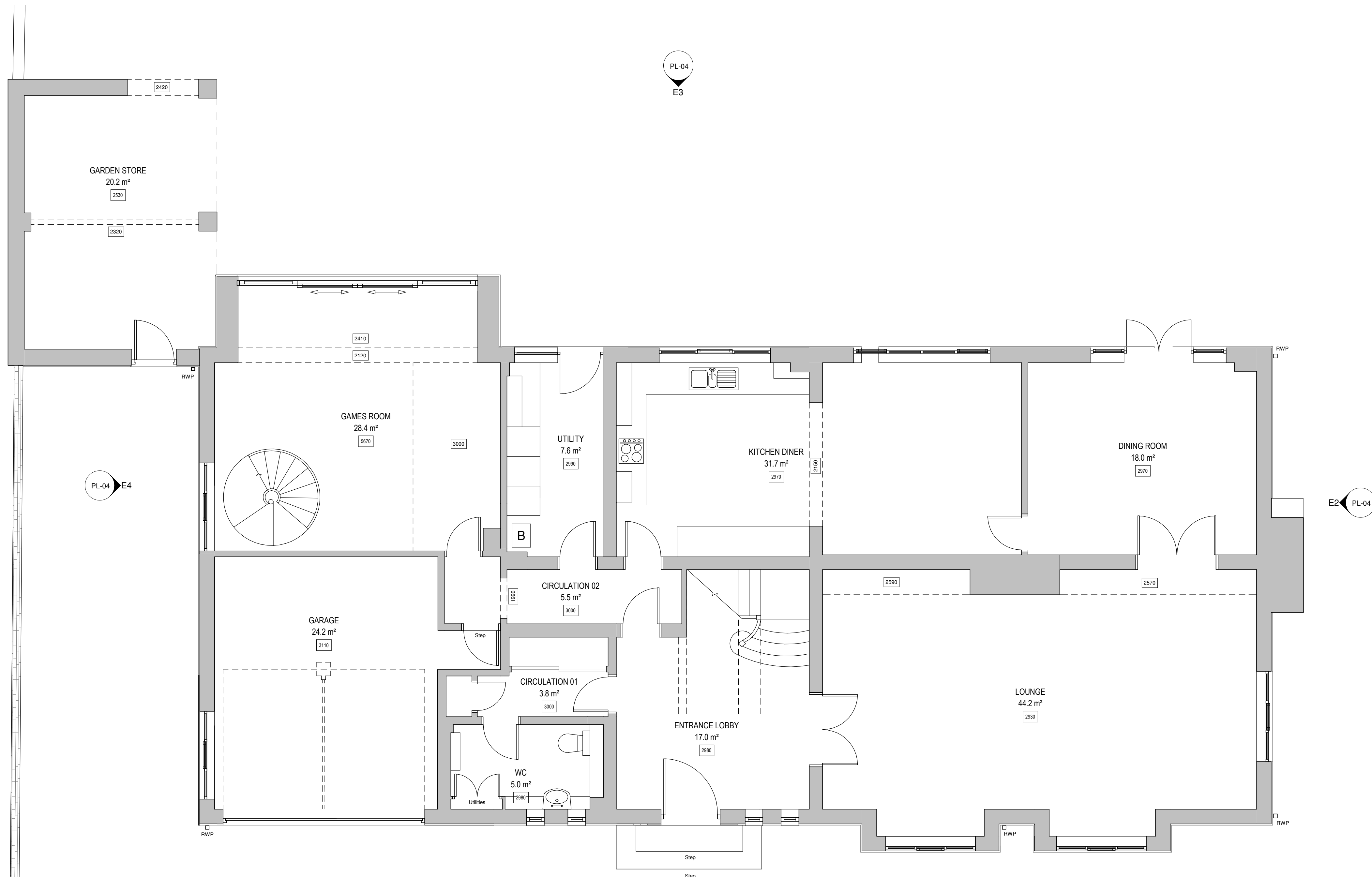
1 Existing Ground Floor Level 1 : 50
