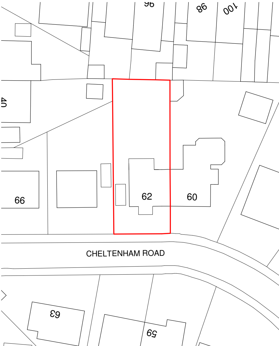
OS Site Plan - Proposed 1 : 500
