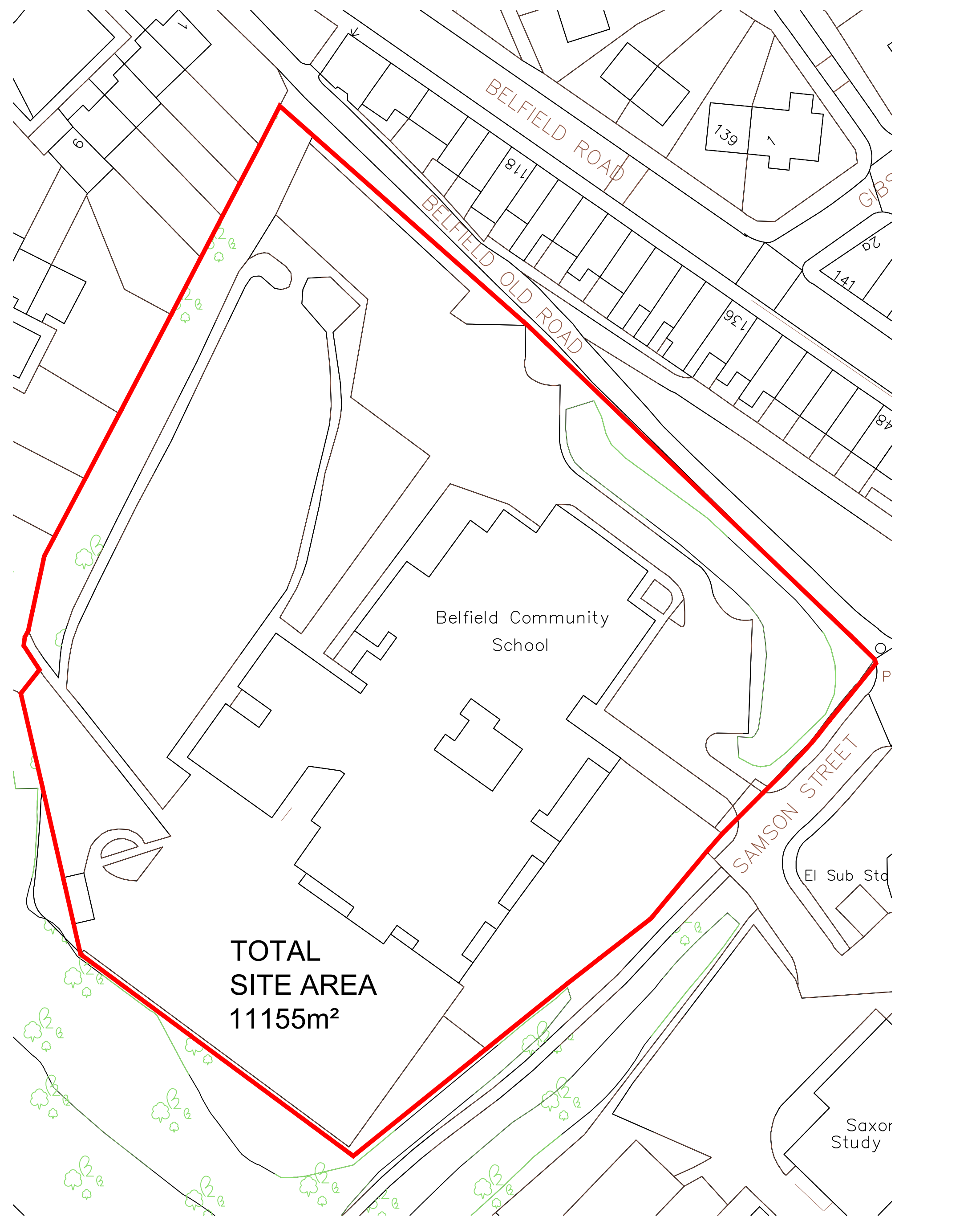
existing and proposed site plan scale 1- 500
