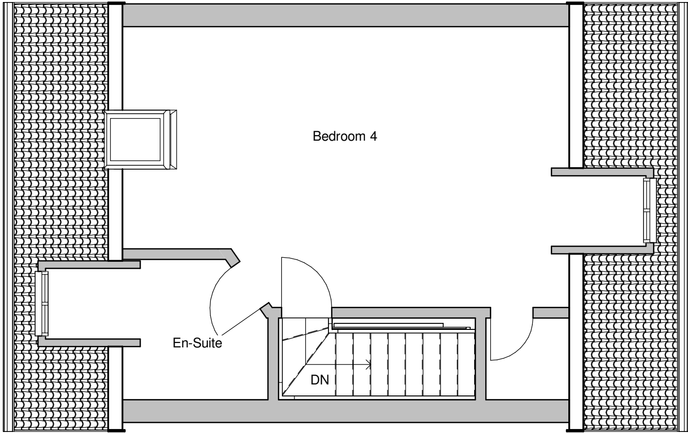
Existing Second Floor 1 : 50
