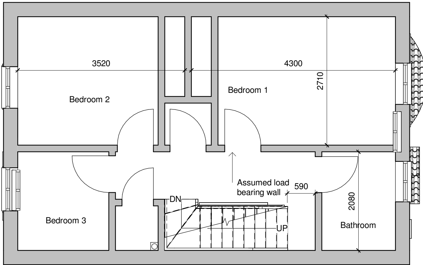
Existing First Floor 1 : 50
