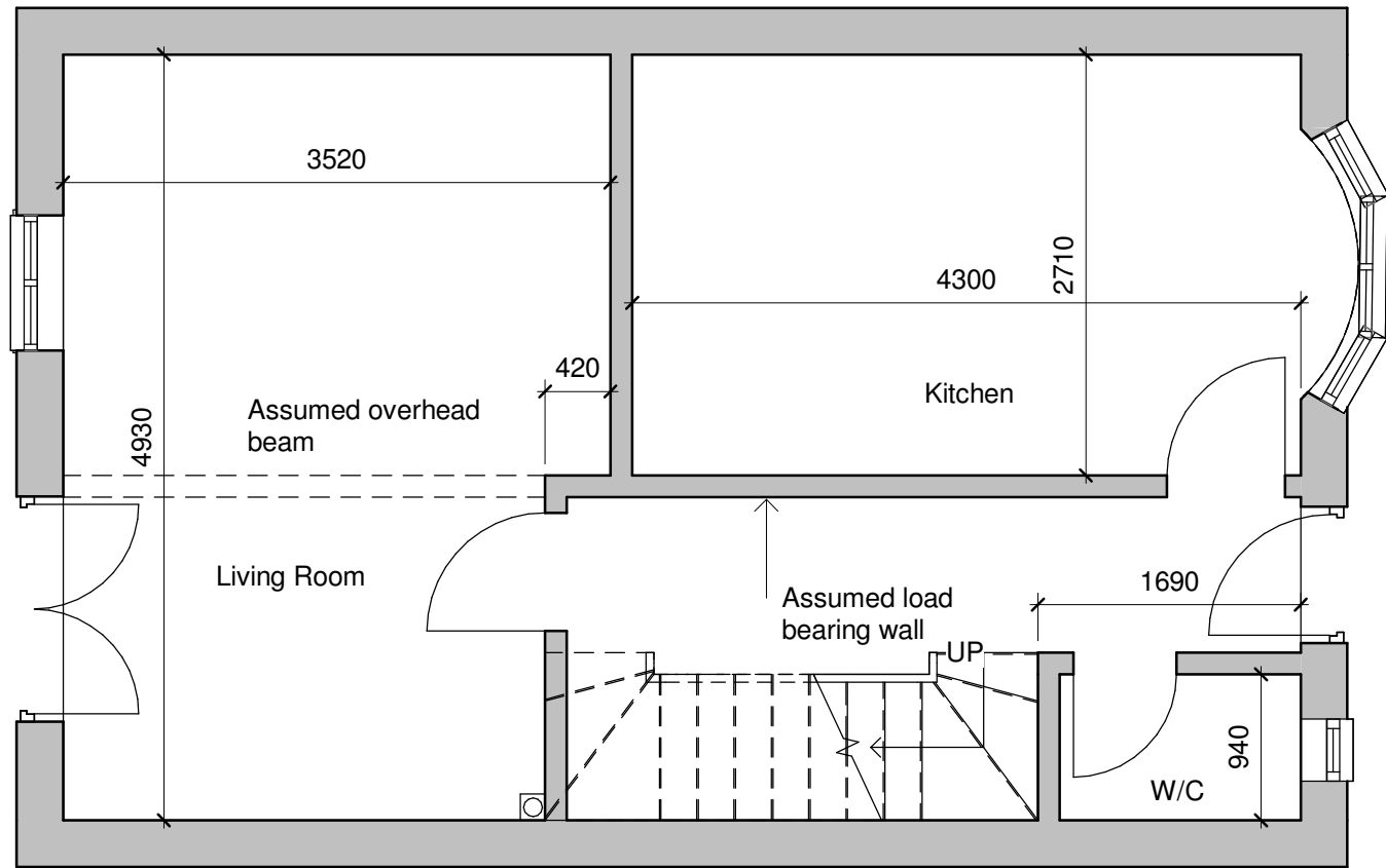
Existing Ground Floor 1 : 50
