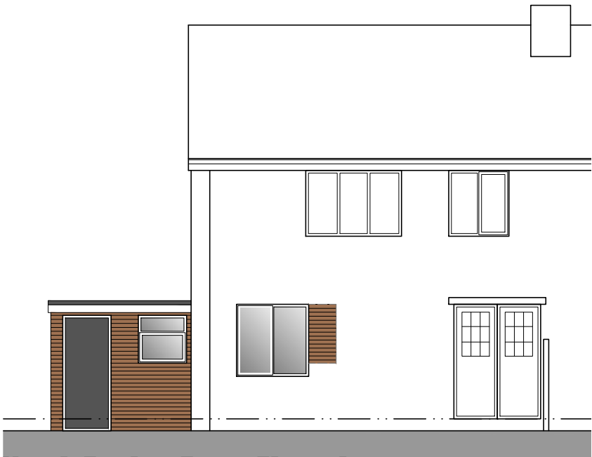
North Facing Front Elevation
