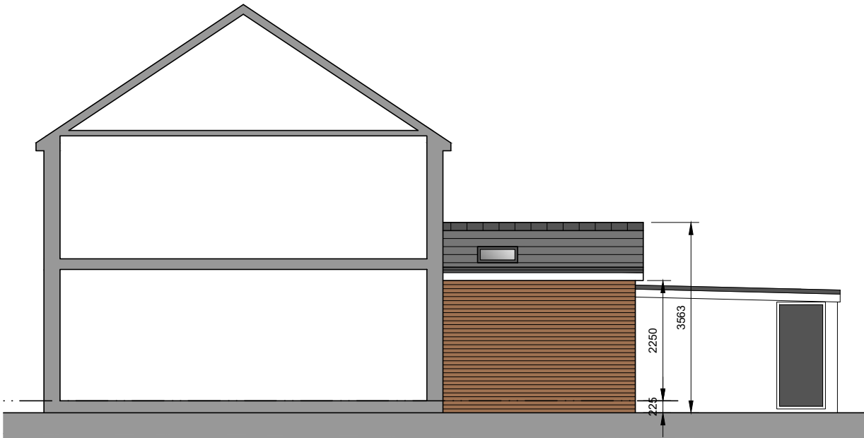
West Facing Side Elevational Section
