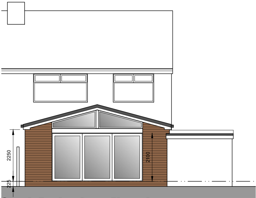
South Facing Rear Elevation
