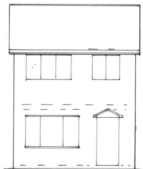
FRONT ELEVATION (EXISTING)
