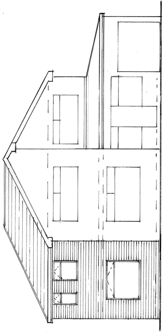
FRONT ELEVATION (PROPOSED)
