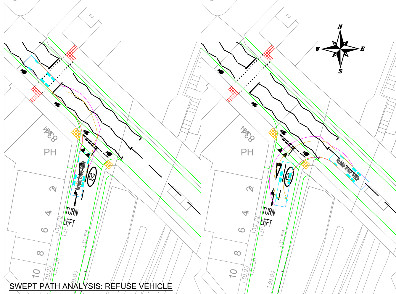
SWEPT PATH ANALYSIS: REFUSE VEHICLE
