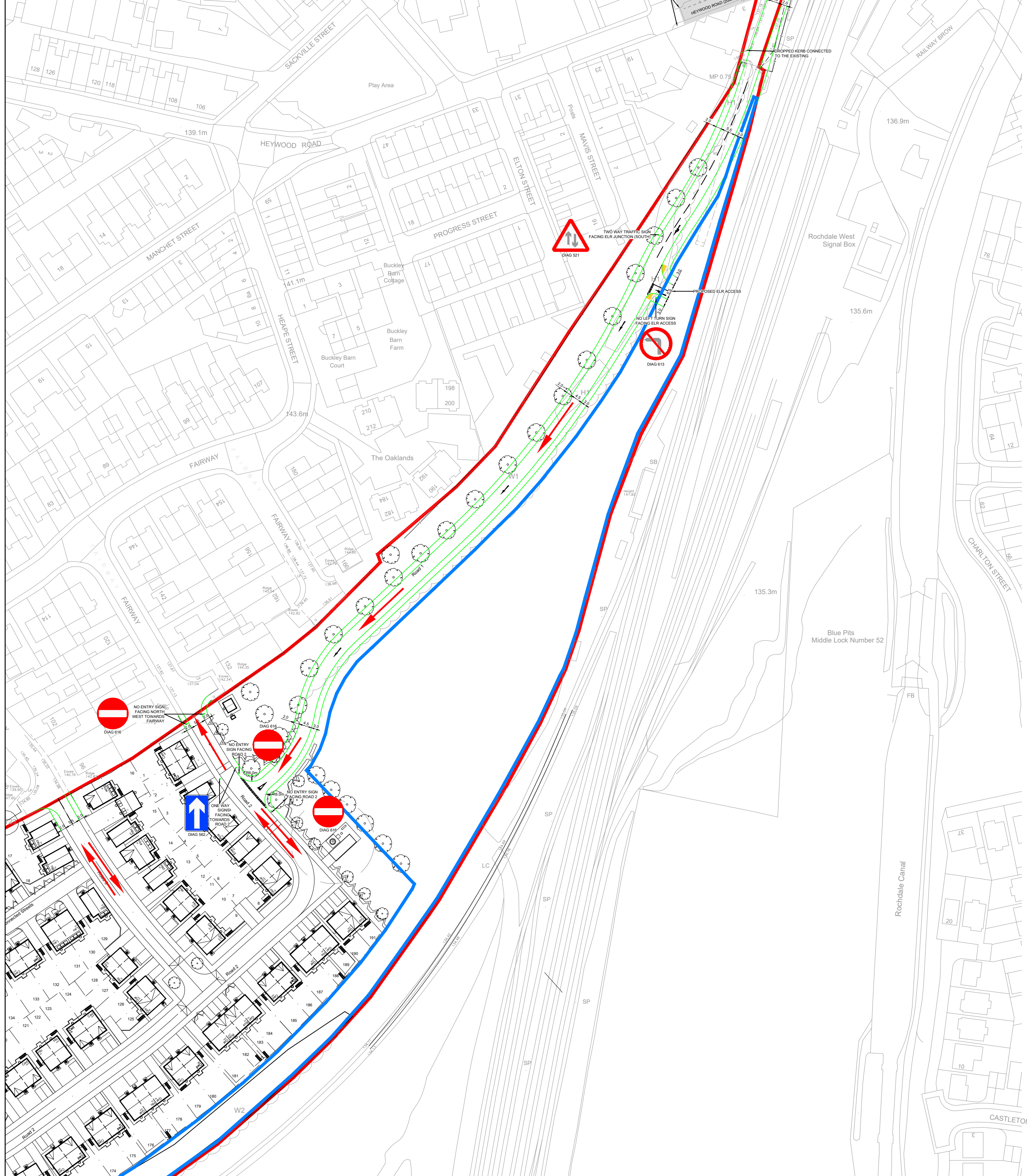
SWEPT PATH ANALYSIS: TIPPER TRUCK
