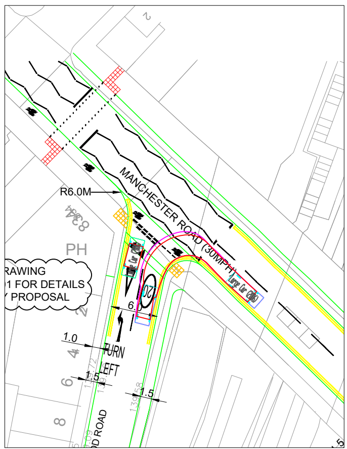
SWEPT PATH ANALYSIS: LARGE CAR
