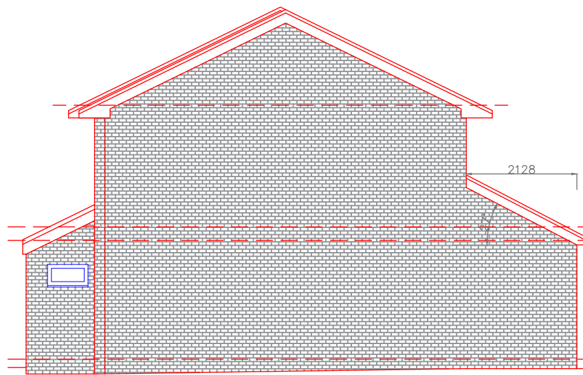
Proposed Side Elevation 1 @1:100
