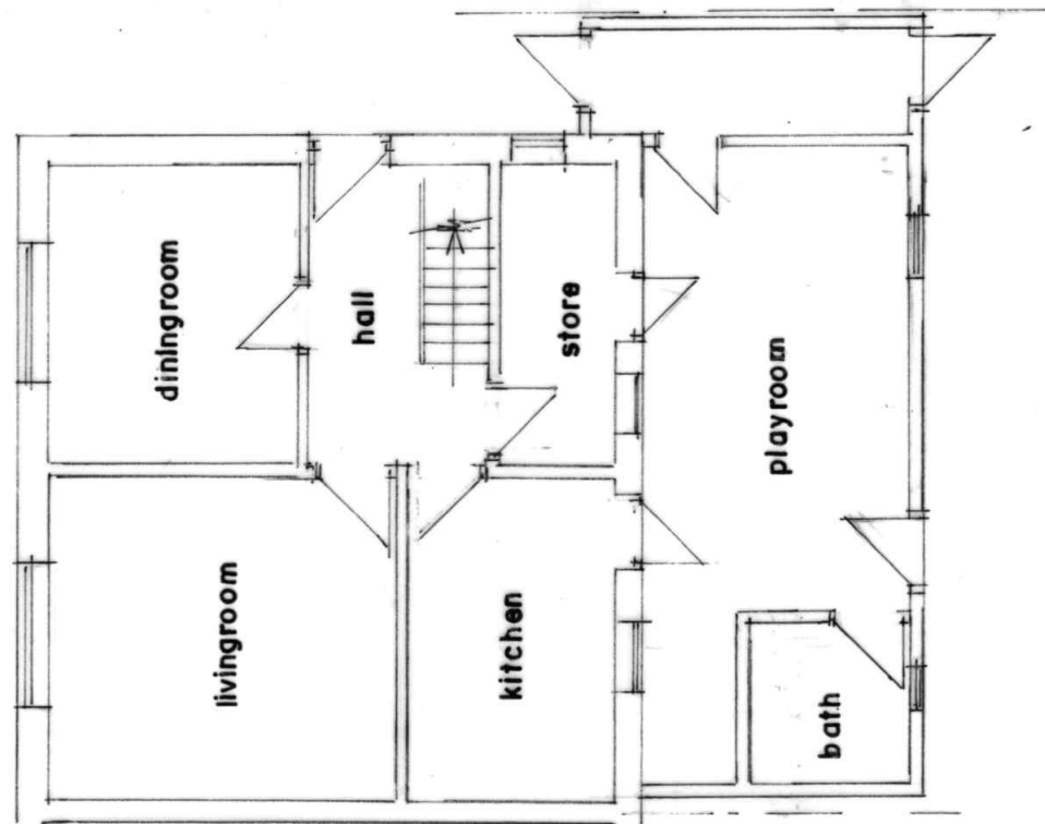
GROUND FLOOR PLAN AFTER
