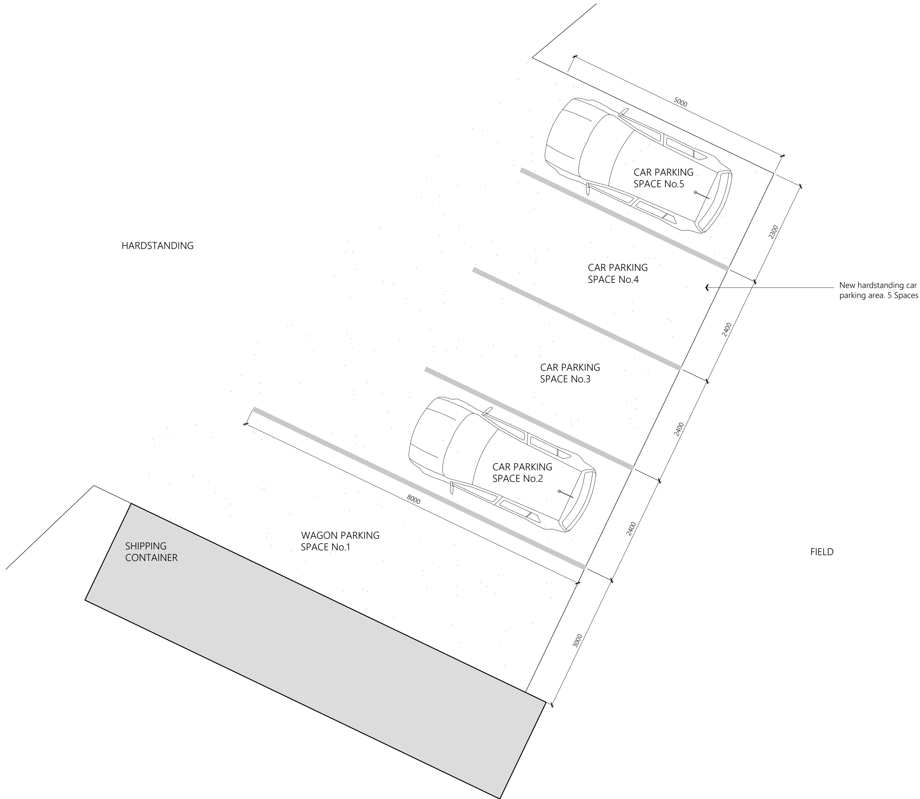
PARKING PLAN
